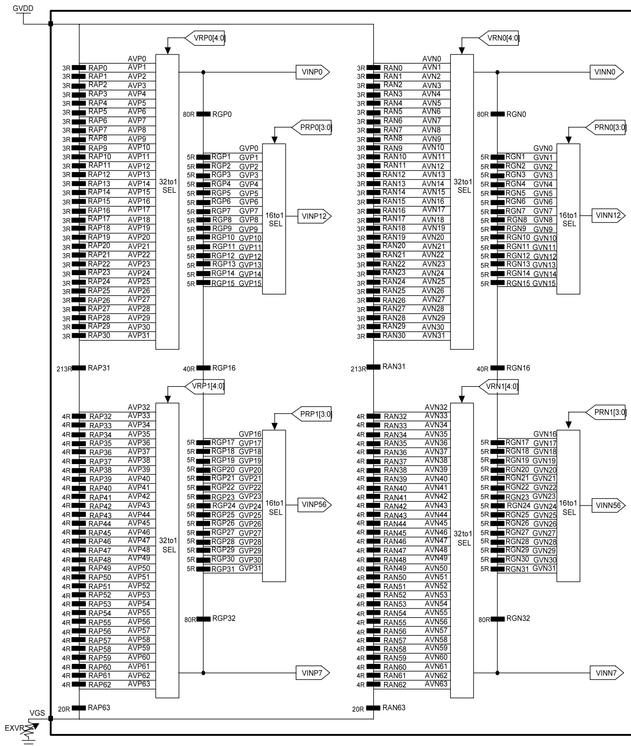
Figure 105 : Structure of Resistor Ladder Network 1
