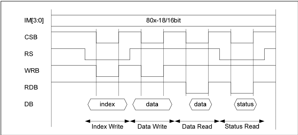
Figure 46 : Timing Diagram of 80-18bit CPU Interface
