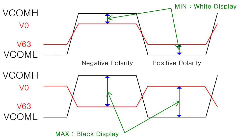
Figure 109 : Relationship Between RAM Data , Source Output Voltage and VCOM (REV=1)
