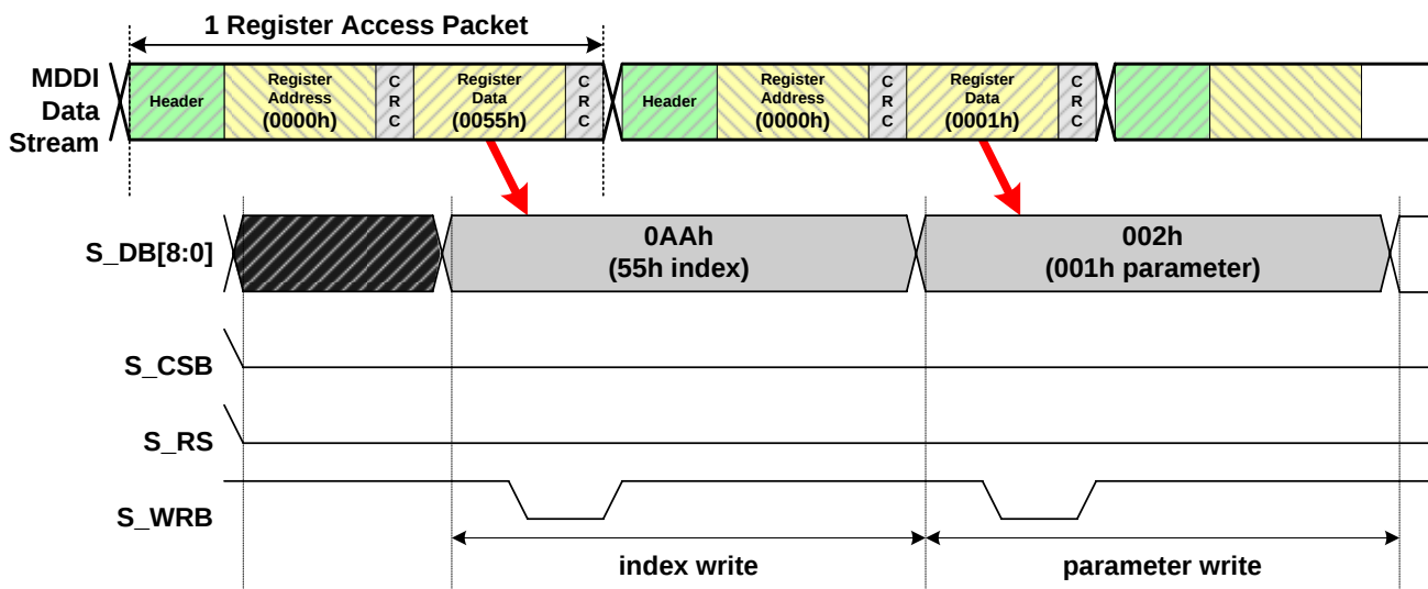
Figure 95 : 80 mode STN type conventional register instruction
