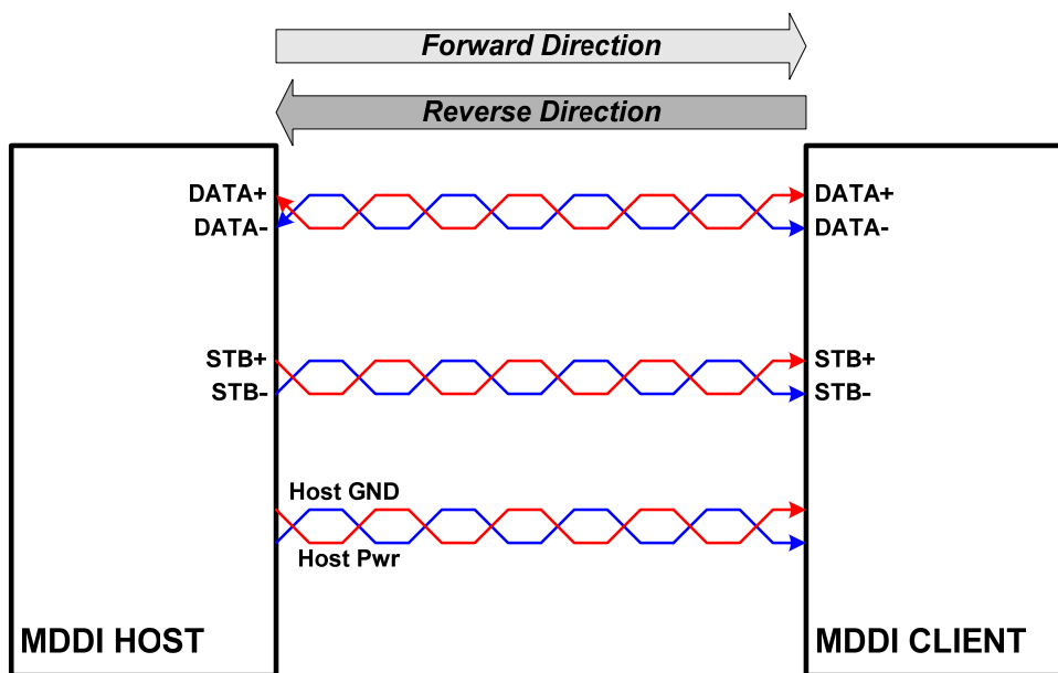
Figure 72 : Physical connection of MDDI host and client
