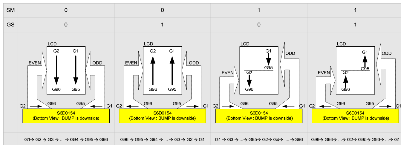
Figure 8 : Gate Clock Generation order selection using GS and SM (NL = 6'b001100, SCN = 6'b000000)
