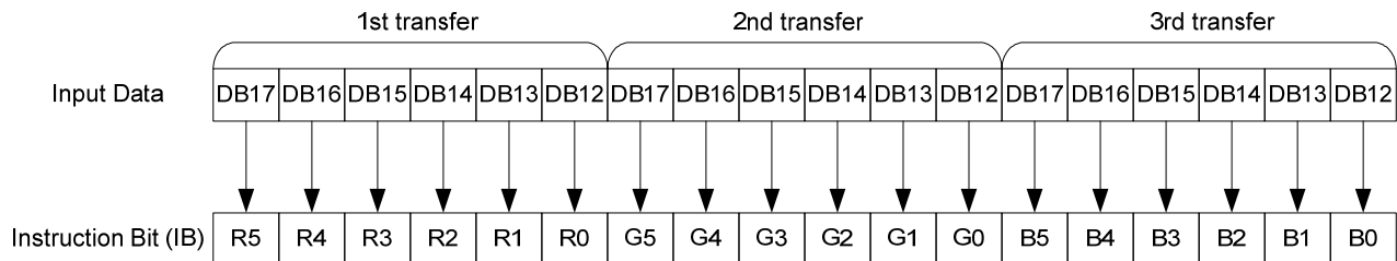
Figure 67 : Bit Assignment of GRAM Data on 6bit RGB Interface
