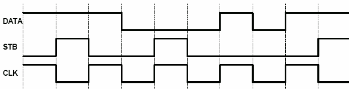
Figure 73 : Data-STB encoding
