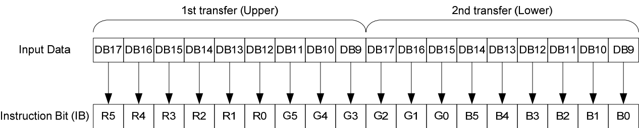
Figure 50 : Bit Assignment of Instructions on 80-9bit CPU Interface
