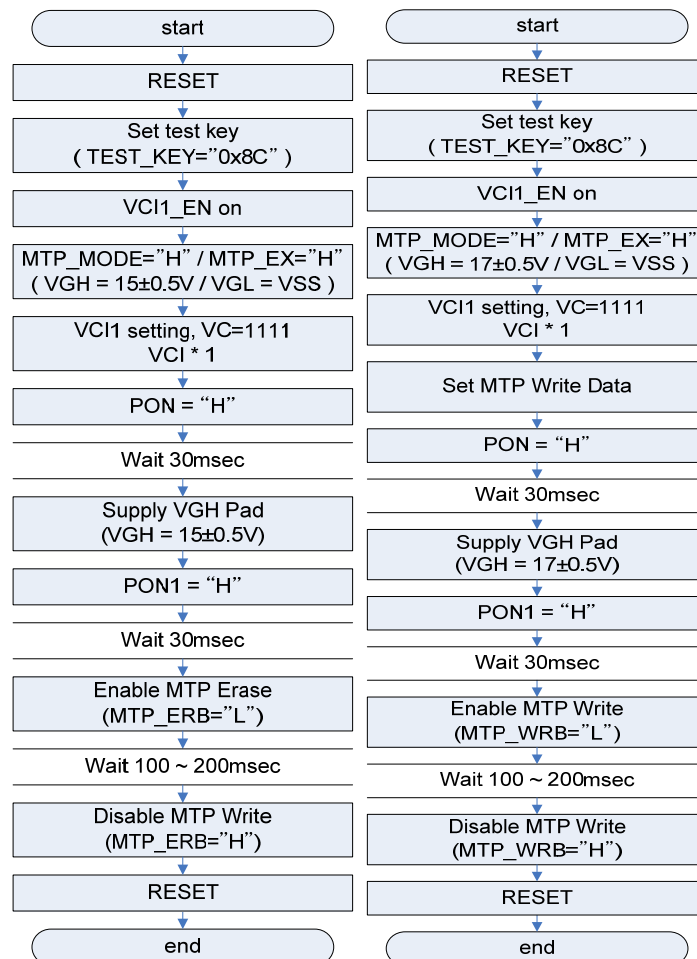
Figure 24 : MTP Initialization, Erase and program
