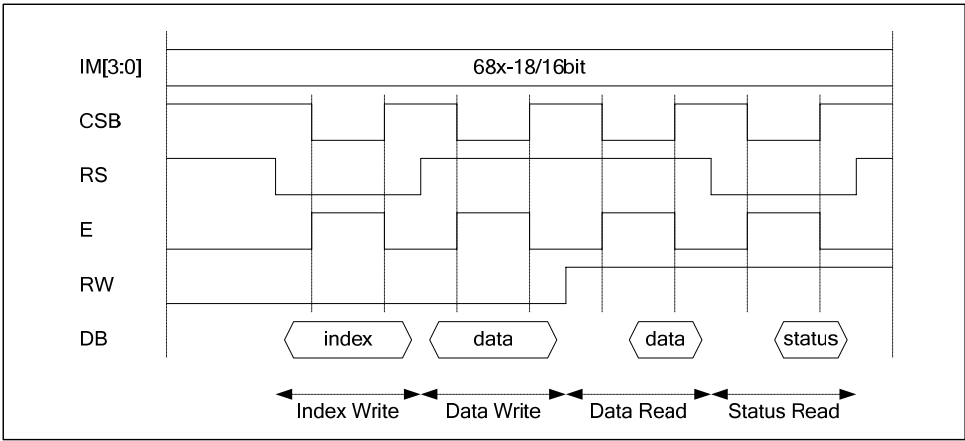
Figure 34 : Timing Diagram of 68-18bit CPU Interface
