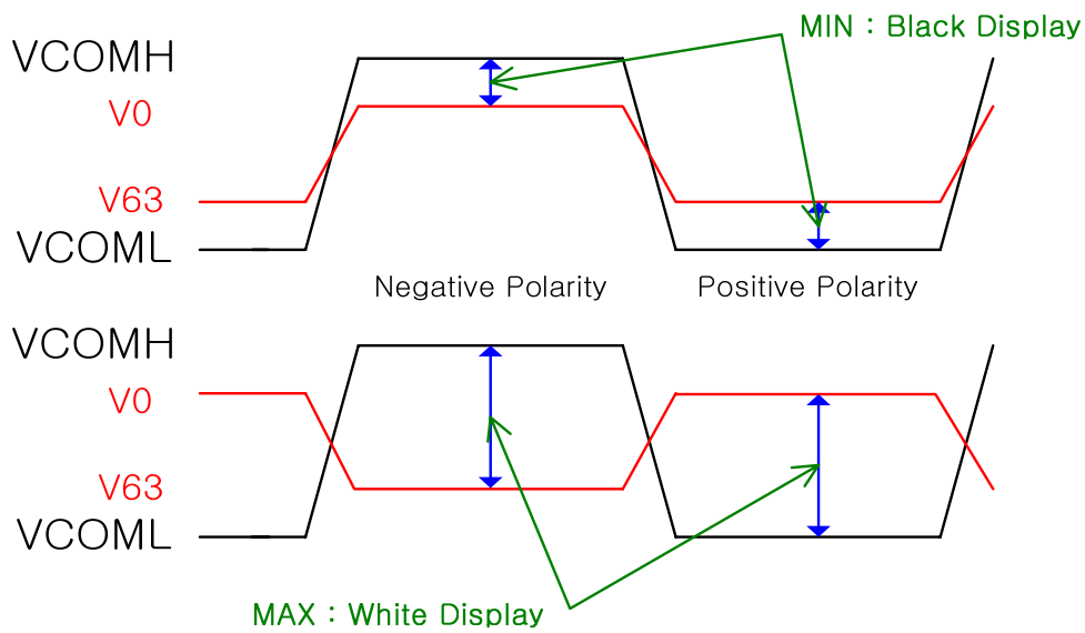
Figure 108 : Relationship Between RAM Data , Source Output Voltage and VCOM (REV=0)
