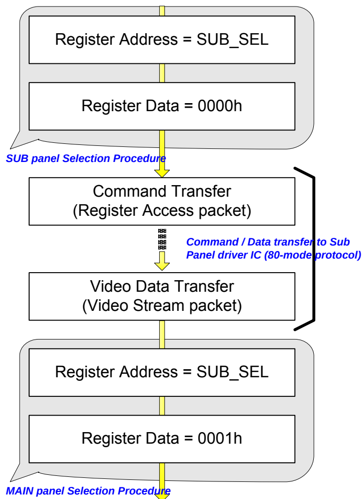
Figure 91 : Main / Sub panel selection procedure
