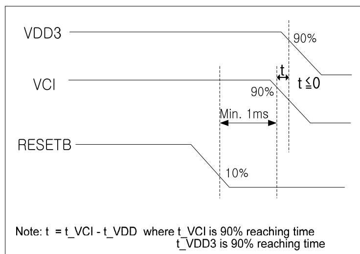
Figure 125 : External Power Off sequence
