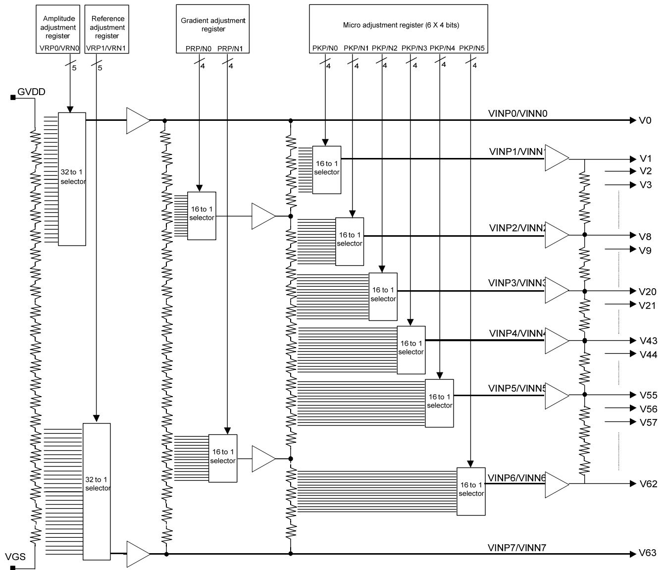
Figure 104 : Structure of Grayscale Amplifier
