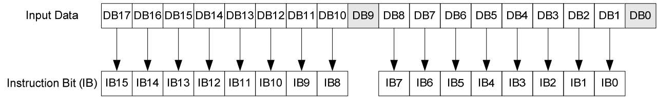
Figure 44 : Bit Assignment of Instructions on 80-18bit CPU Interface
