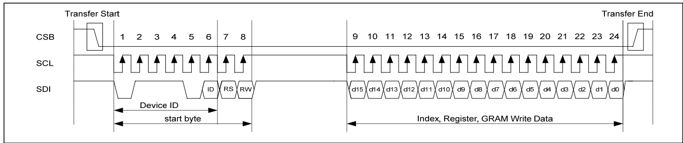
Figure 58 : Basic Timing Diagram of Data Transfer through SPI
