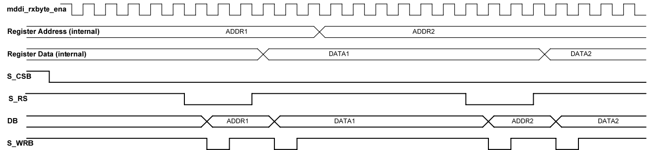
Figure 99 : Index/parameter write timing diagram
