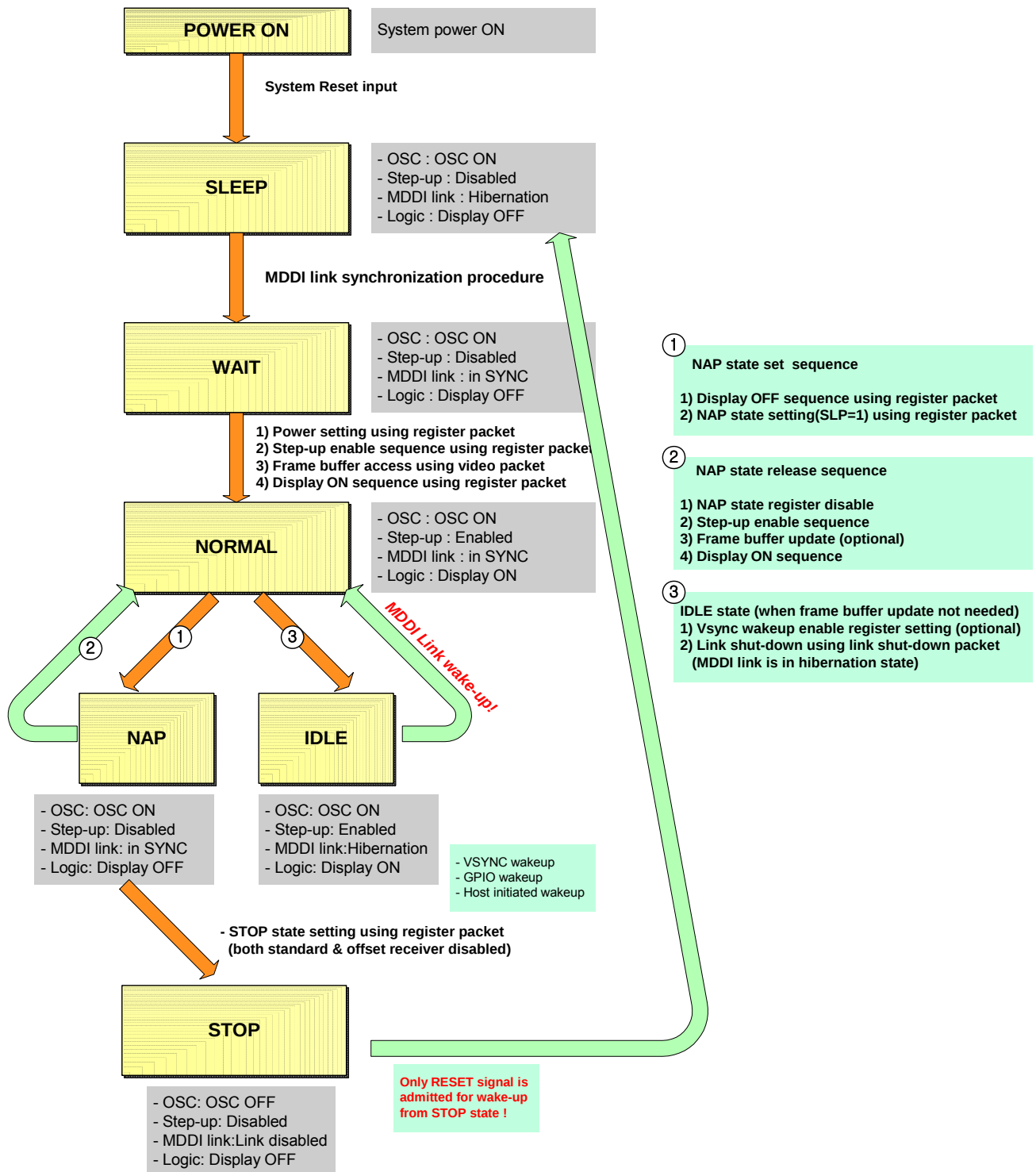
Figure 89 : Operating state in MDDI mode
