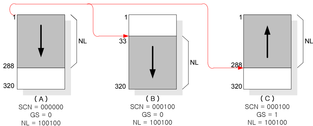
Figure 17 : Gate Scan Position Control
