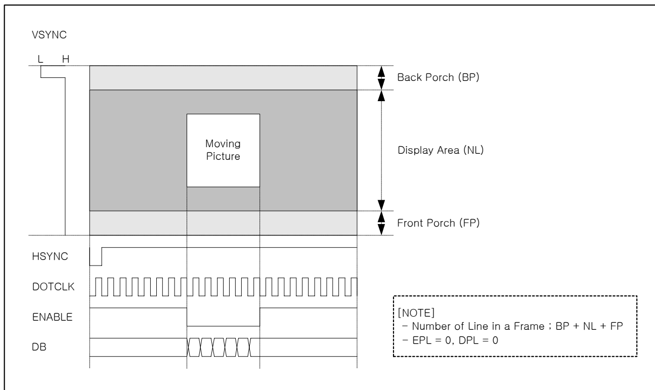
Figure 62 : RGB Interface
