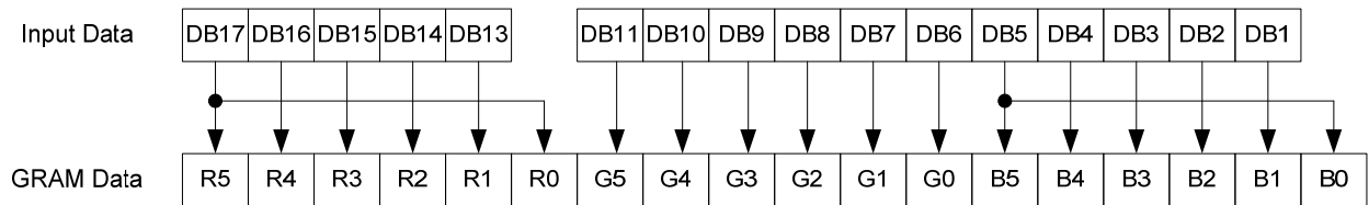
Figure 65 : Bit Assignment of GRAM Data on 16bit RGB Interface
