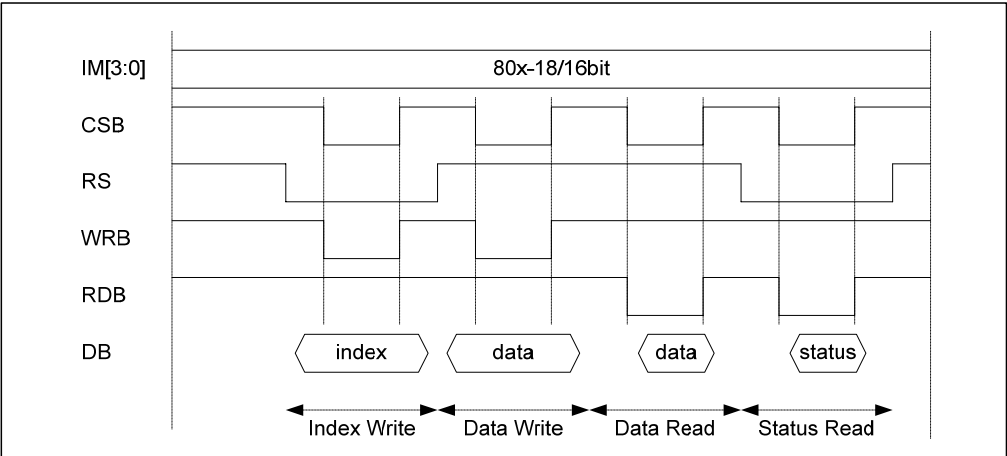
Figure 49 : Timing Diagram of 80-16bit CPU Interface
