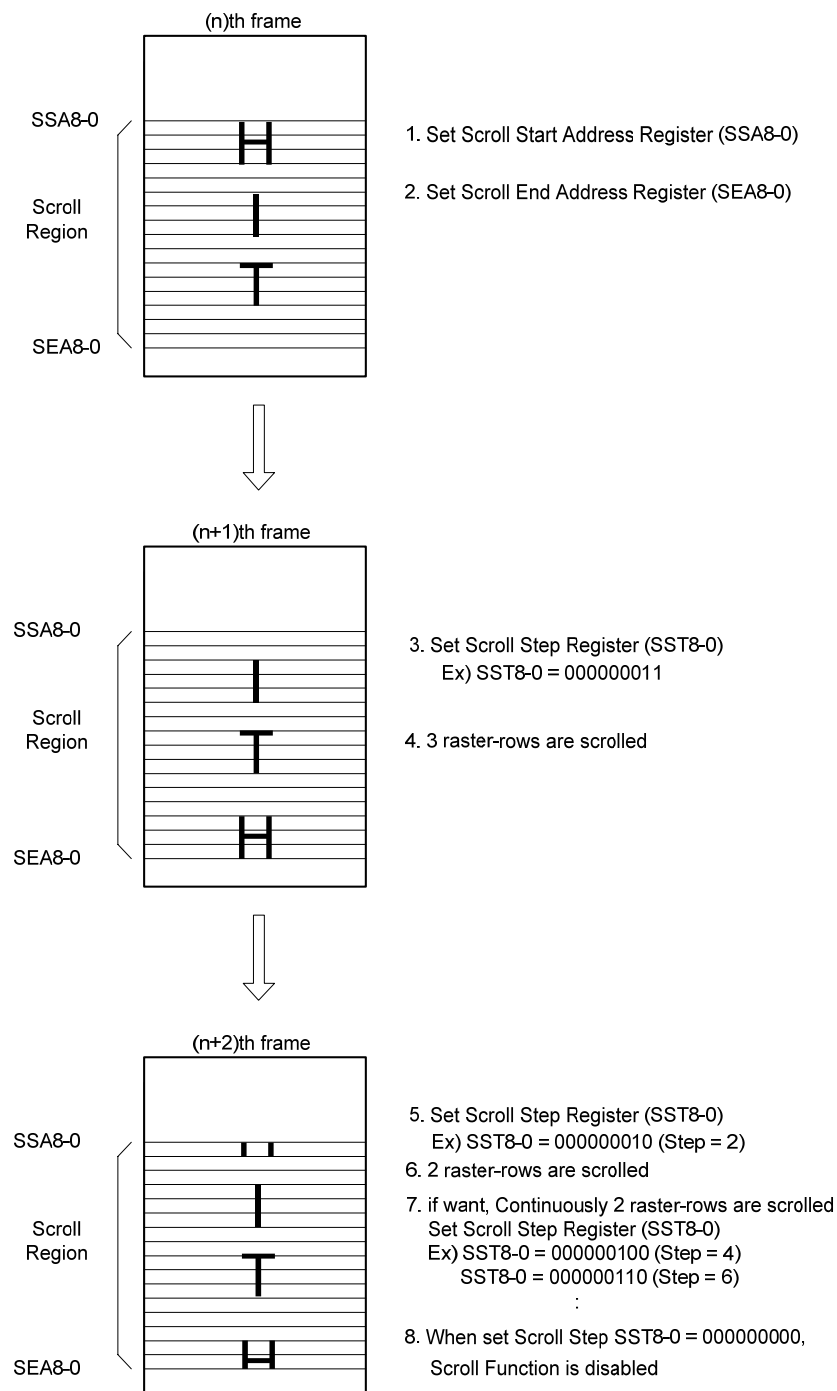
Figure 18 : Vertical Scroll Display
