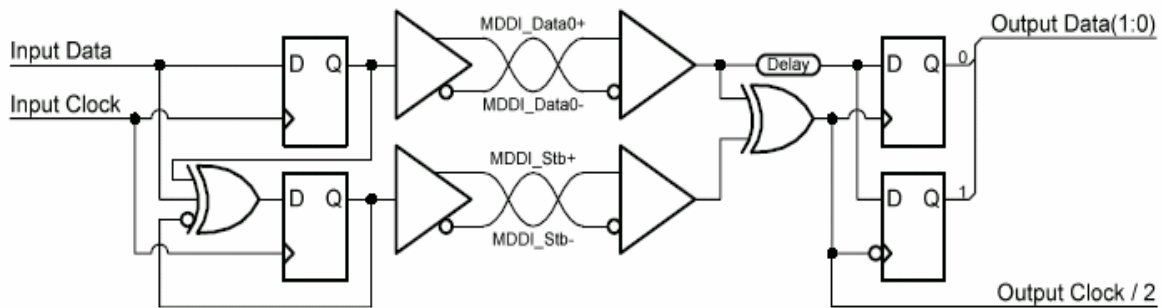
Figure 74 : Data / STB Generation & Recovery circuit
