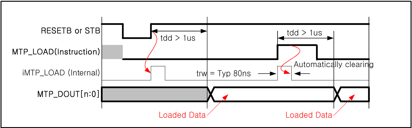
Figure 26 : Timing of MTP Load
