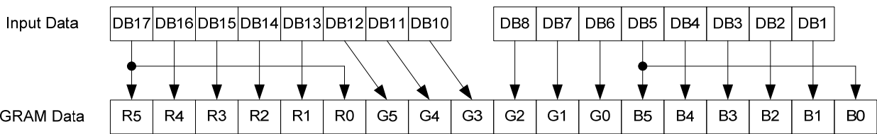
Figure 47 : Bit Assignment of Instructions on 80-16bit CPU Interface
