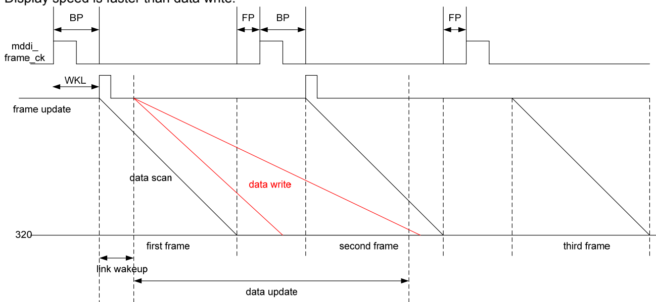
Figure 83 : Tearing-less display: display speed is faster than data write
