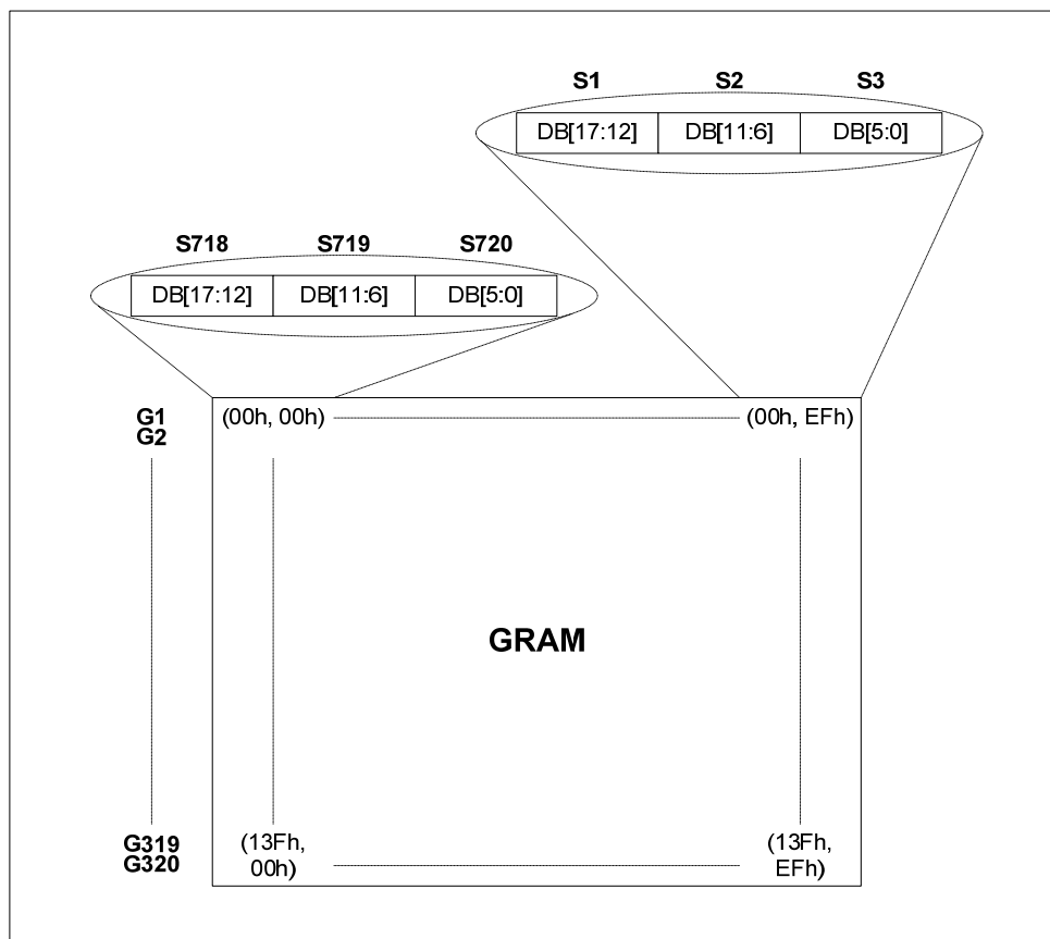
Figure 9 : Image mirroring using SS register (SS = "1")
