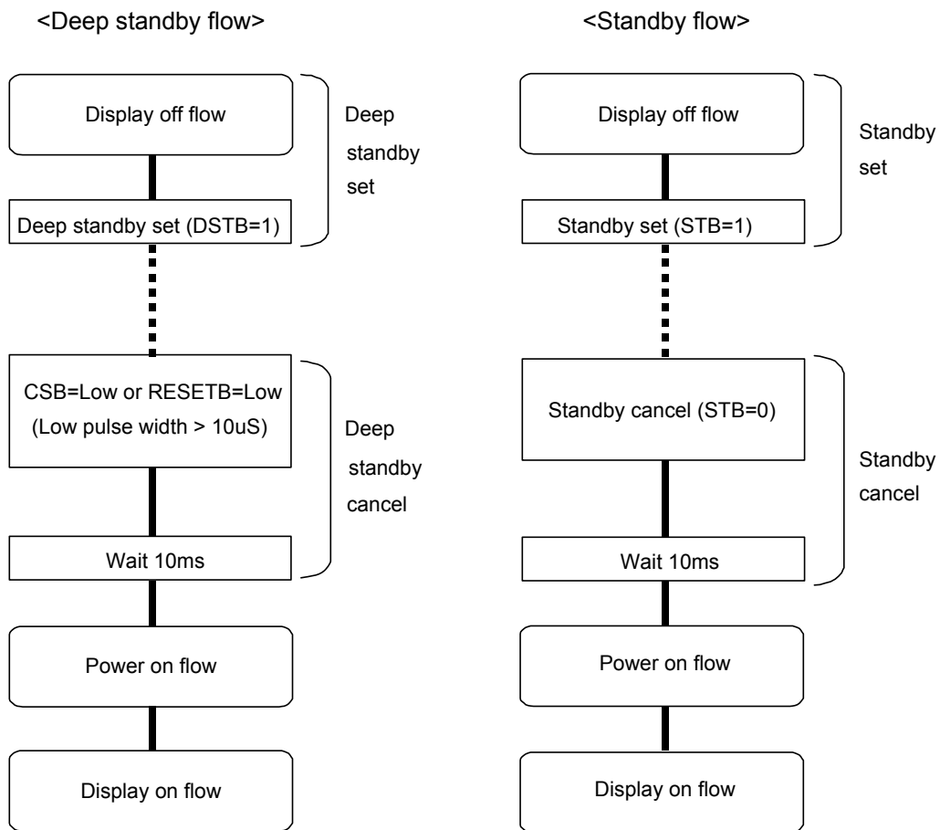
Figure 113 : D-STAND-BY/STAND-BY SEQUENCE
