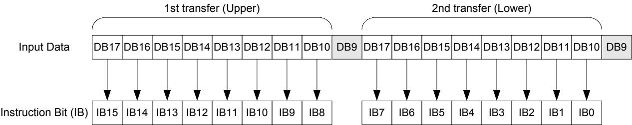
Figure 38 : Bit Assignment of Instructions on 68-9bit CPU Interface
