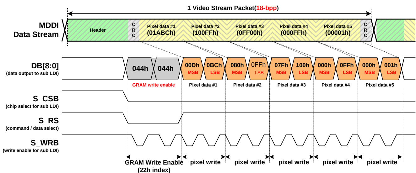
Figure 93 : 80 mode 9 bit video data transfer
