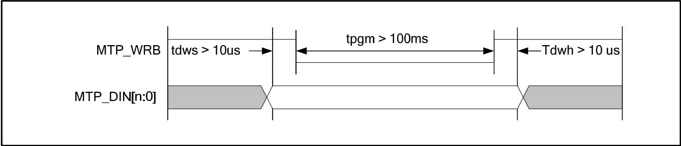
Figure 25 : Timing of MTP Program
