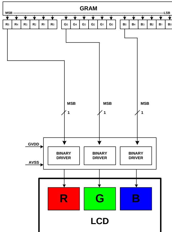
Figure 110 : 8-Color Display Control
