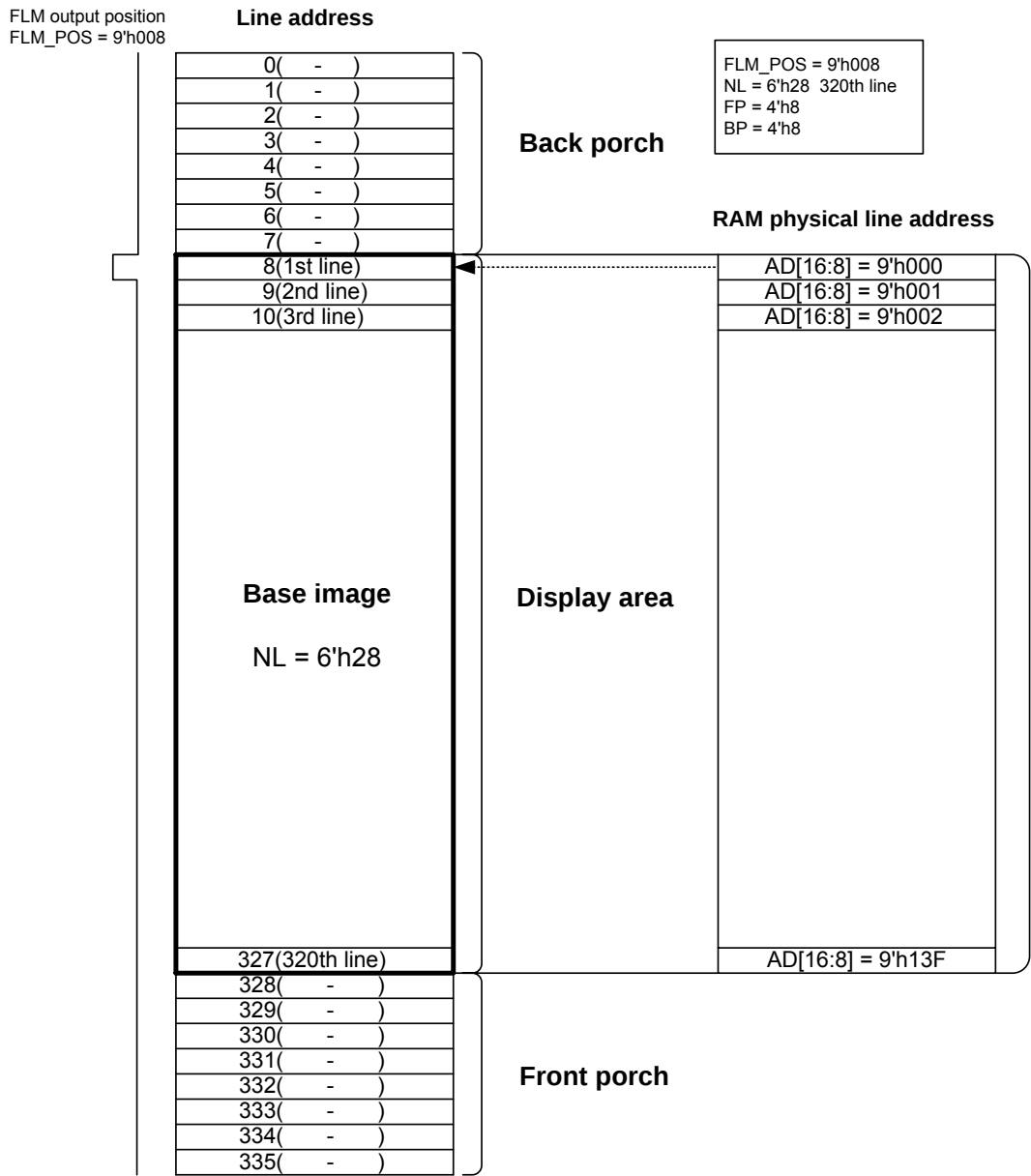
Figure 16 : FLM_POS Setting
