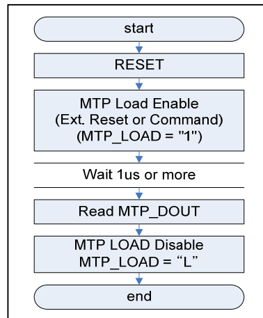
Figure 23 : Flow of MTP Load / Read
