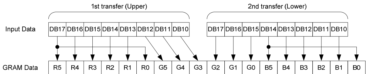
Figure 41 : Bit Assignment of Instructions on 68-8bit CPU Interface
