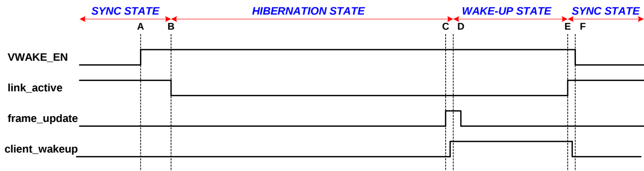
Figure 87 : VSYNC based link wake-up procedure
