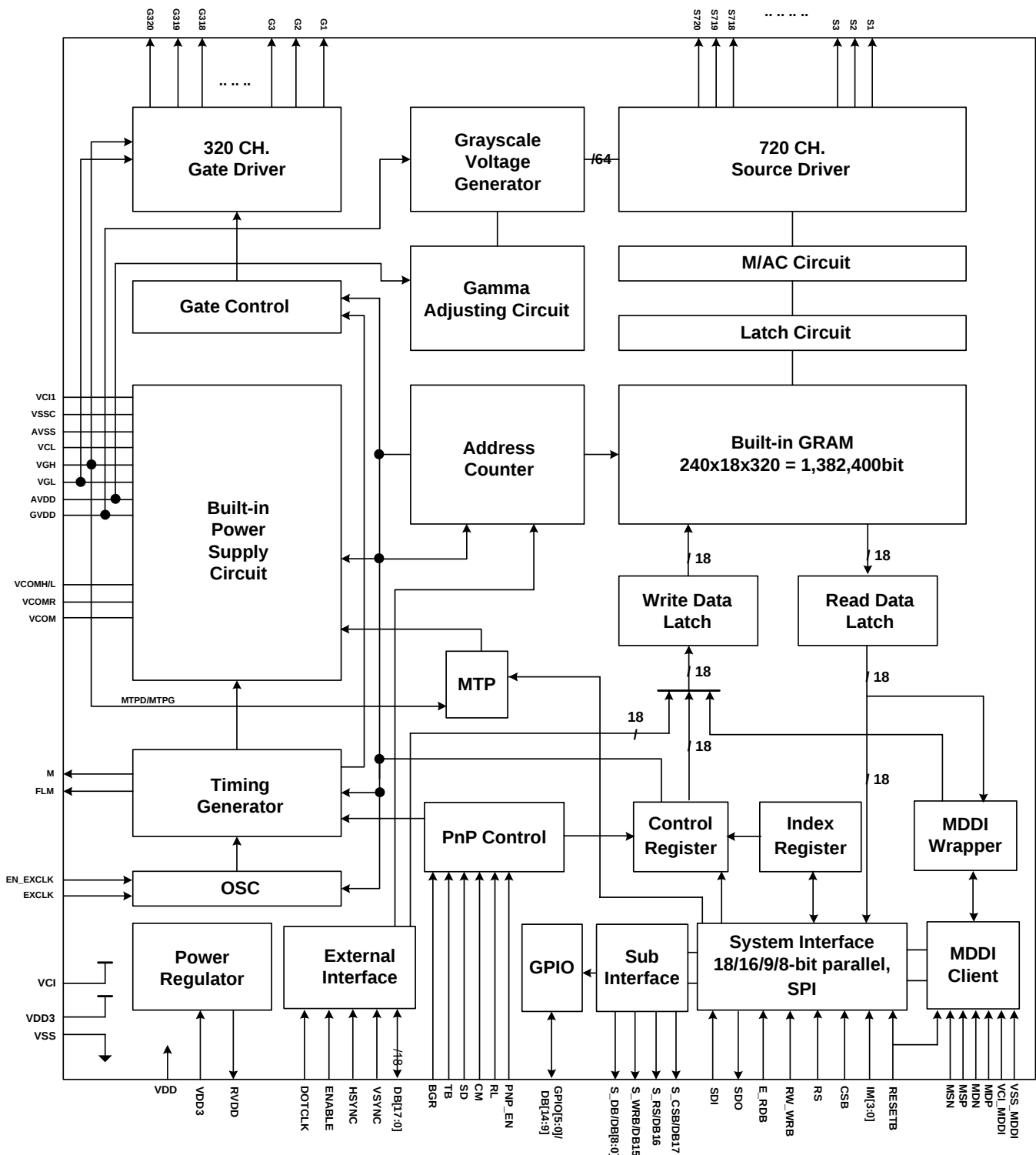
Figure 1 : Block Diagram of S6D0154
