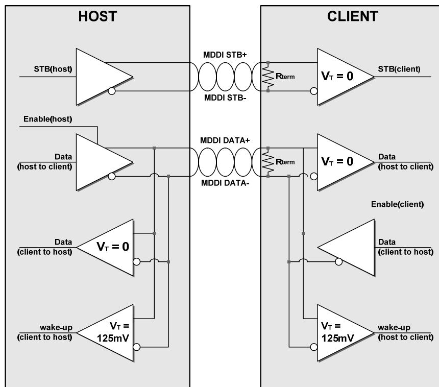
Figure 75 : Differential connection between host and client
