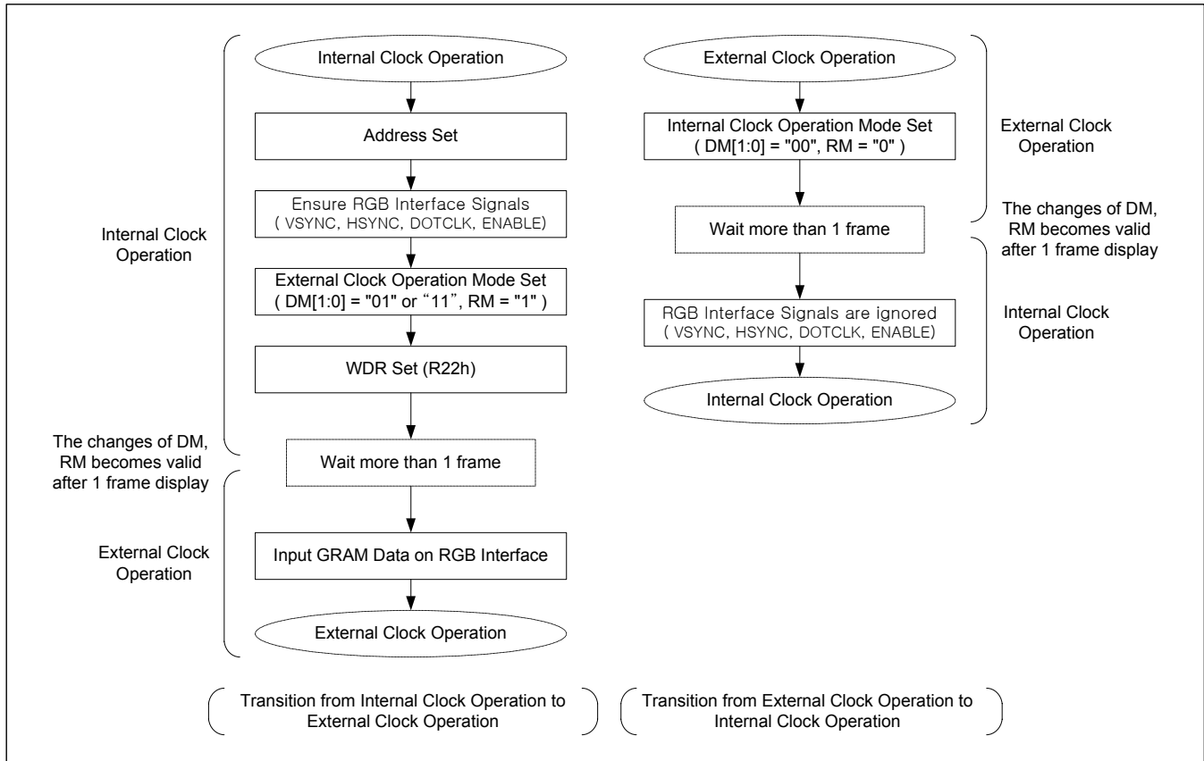
Figure 71 : Transition between Internal Clock Operation Mode and External Clock Operation Mode
