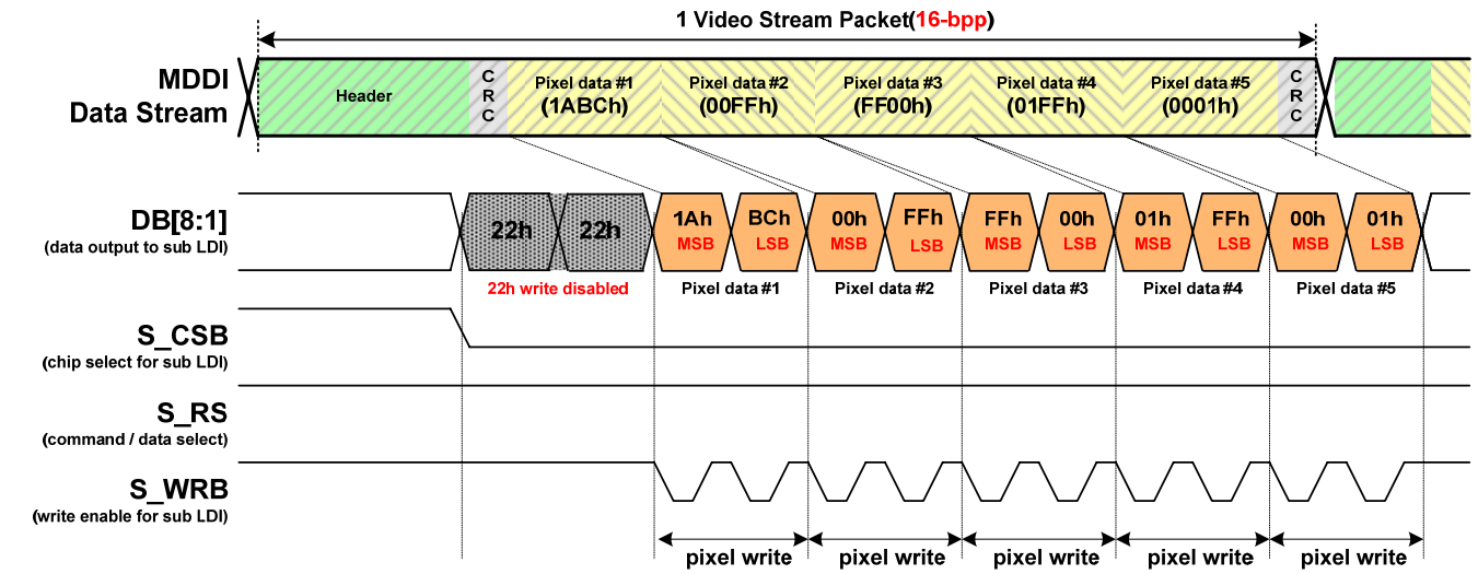
Figure 98 : 80 mode STN type 8bit video data transfer
