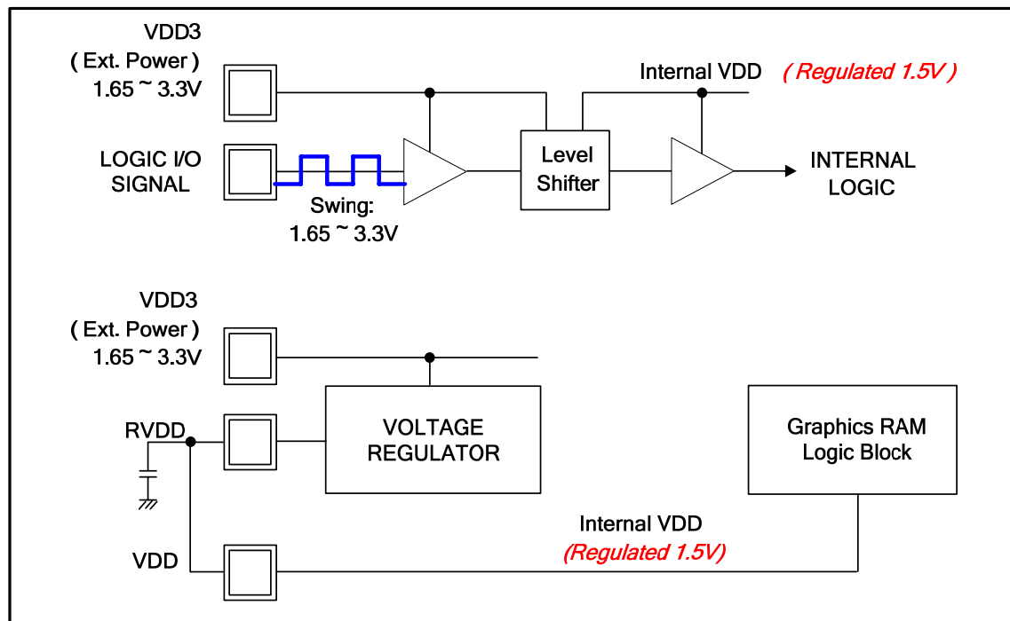
Figure 30 : Voltage Regulation Function
