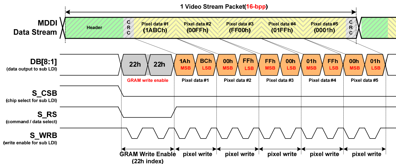
Figure 94 : 80 mode 8 bit video data transfer
