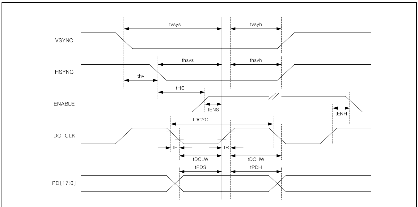
Figure 122 : AC Characteristics (RGB Interface Mode)
