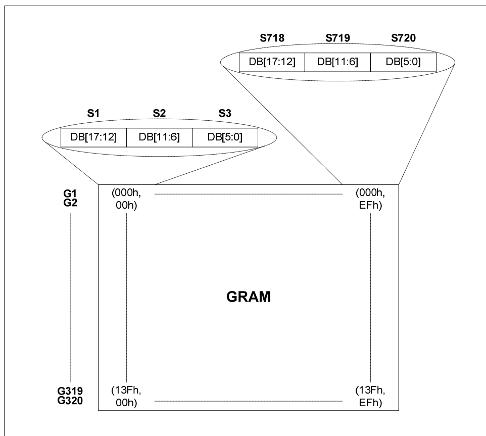
Figure 3 : GRAM Address and Display Image
