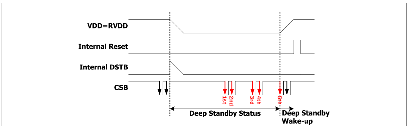
Figure 114 : DEEP STAND-BY EXIT FLOW
