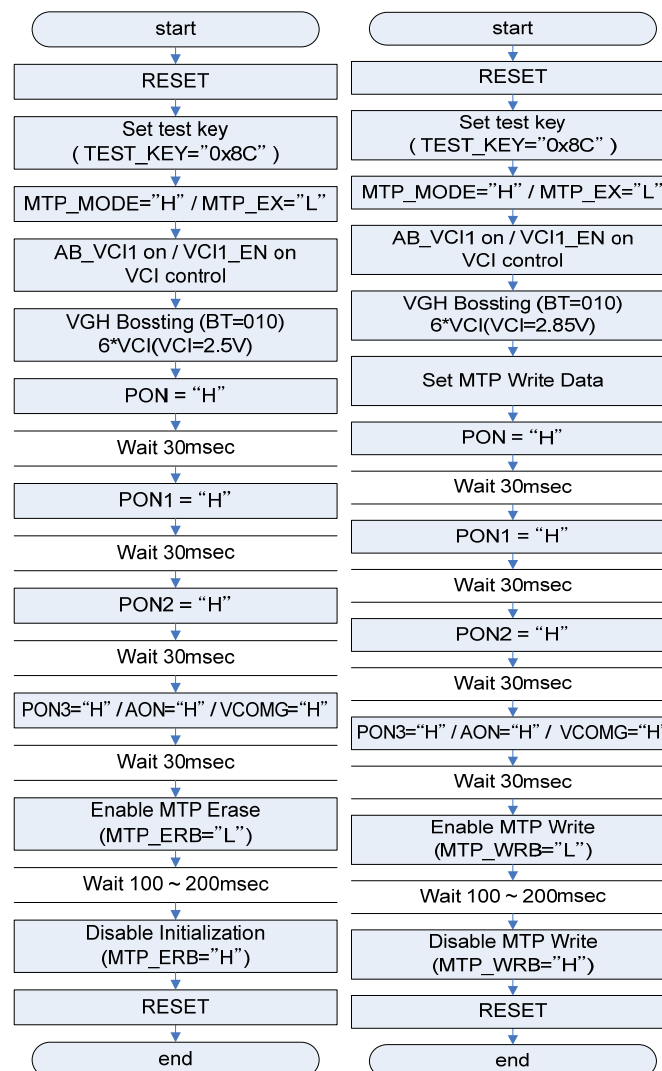
Figure 22 : MTP Initialization, Erase and program
