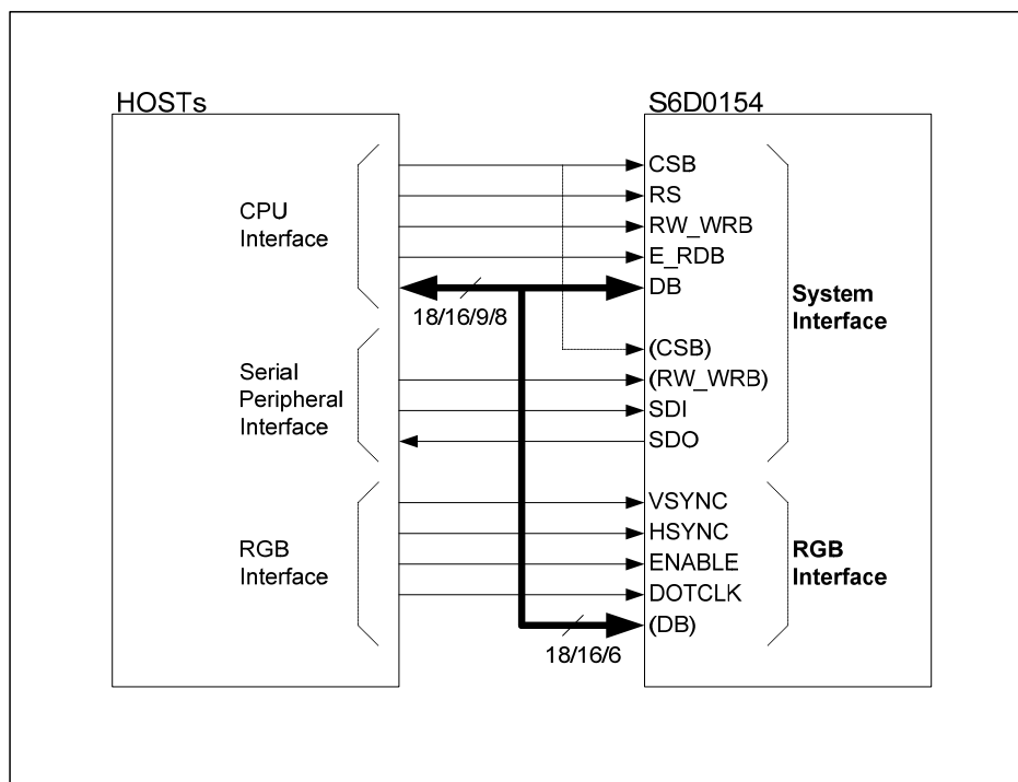
Figure 31 : System Interface and RGB Interface
