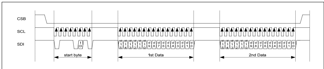
Figure 59 : Timing Diagram of Consecutive Data-Write through SPI
