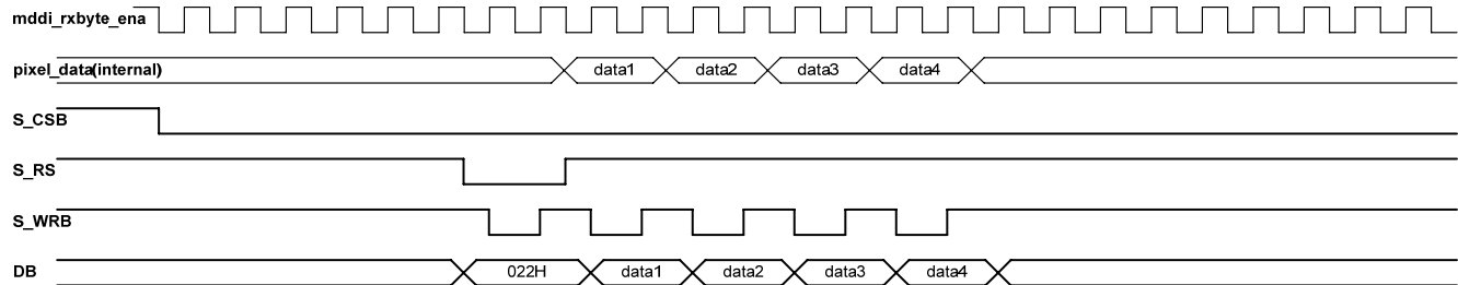
Figure 100 : Image data write timing diagram
