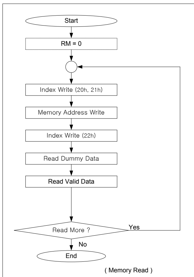
Figure 15 : Memory Data Read Sequence
