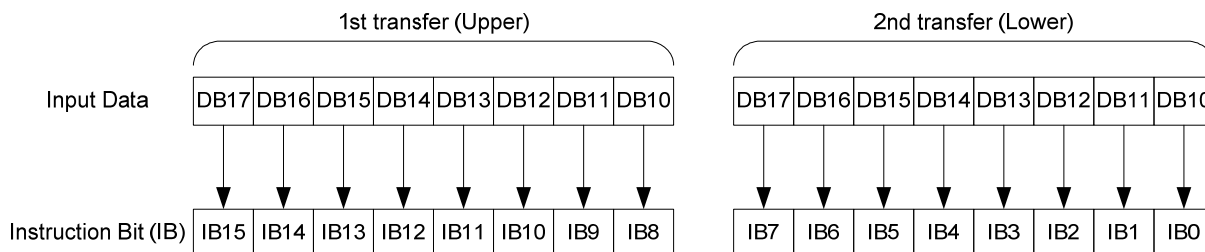
Figure 53 : Bit Assignment of Instructions on 80-8bit CPU Interface
