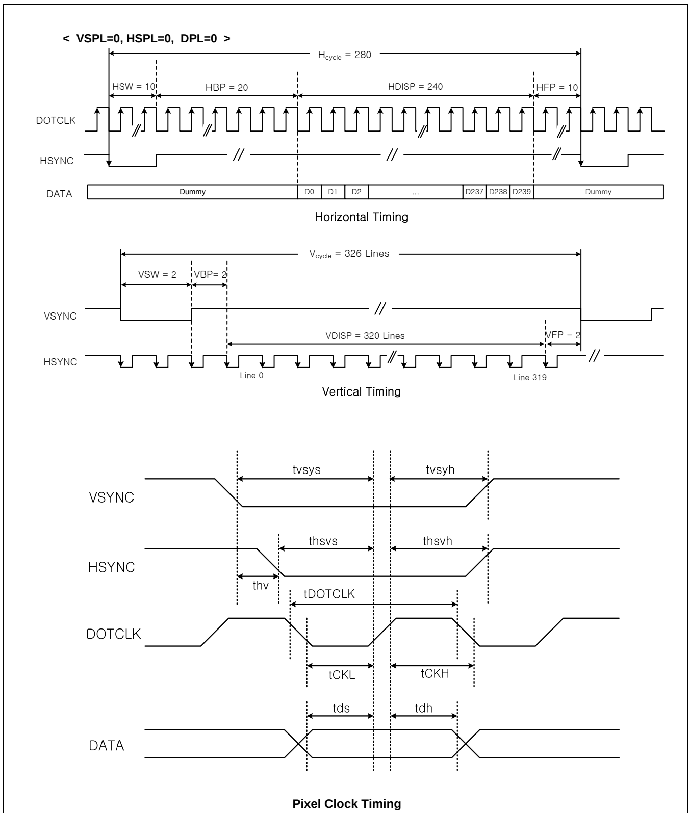
Figure 4 : Plug & Play Timing Diagram
