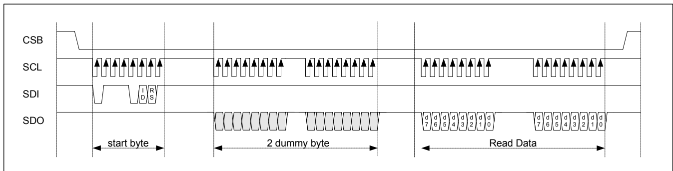
Figure 60 : Timing Diagram of Register / Status Read through SPI
