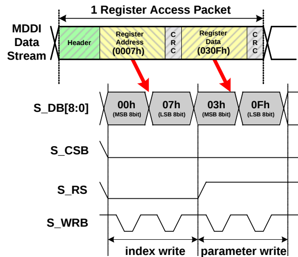
Figure 92 : 80mode 9/8 bit type register access data transfer
