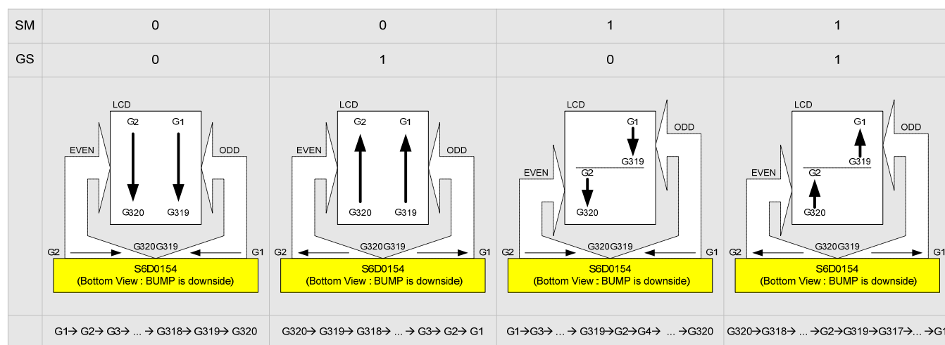
Figure 7 : Gate Clock Generation order selection using GS and SM (NL = 6'b101000, SCN = 6'b000000)
