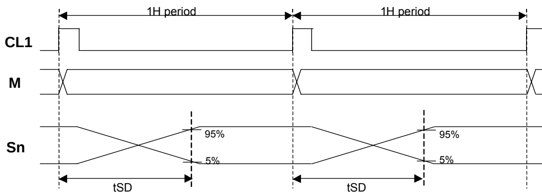
Figure 118 : LCD source driver delay
