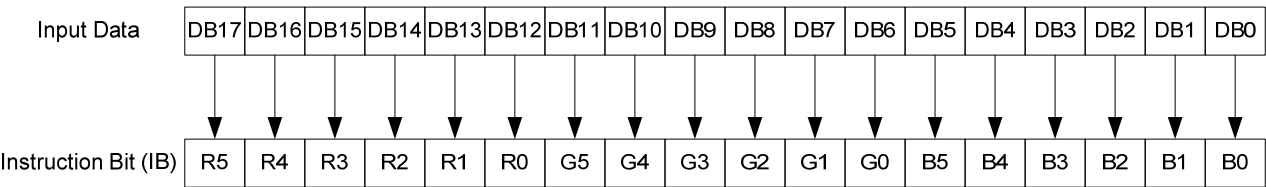
Figure 32 : Bit Assignment of Instructions on 68-18bit CPU Interface
