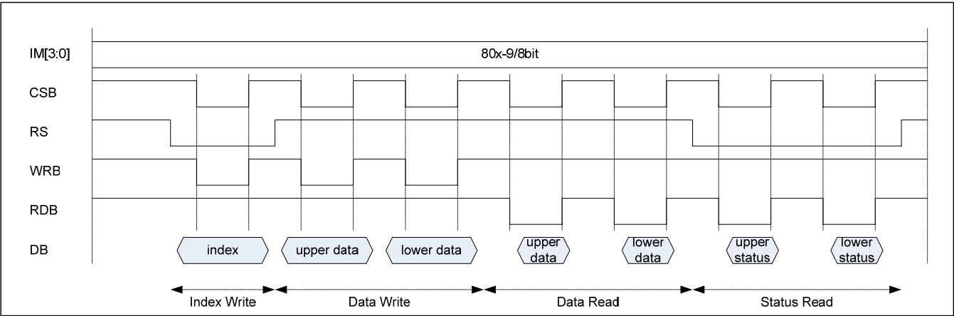
Figure 52 : Timing Diagram of 80-9bit CPU Interface
