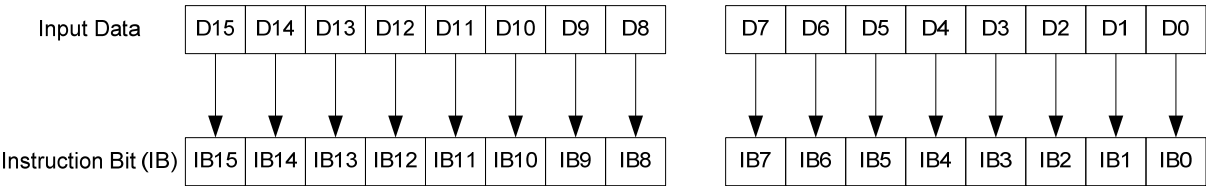
Figure 56 : Bit Assignment of Instructions on SPI
