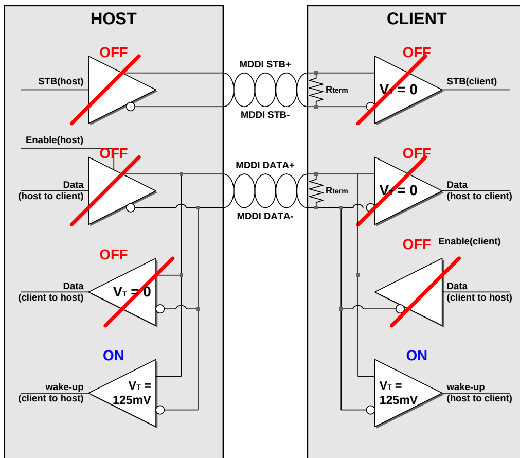
Figure 84 : MDDI Transceiver / Receiver state in hibernation
