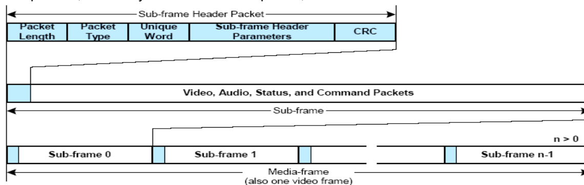
Figure 76 : MDDI packet structure
