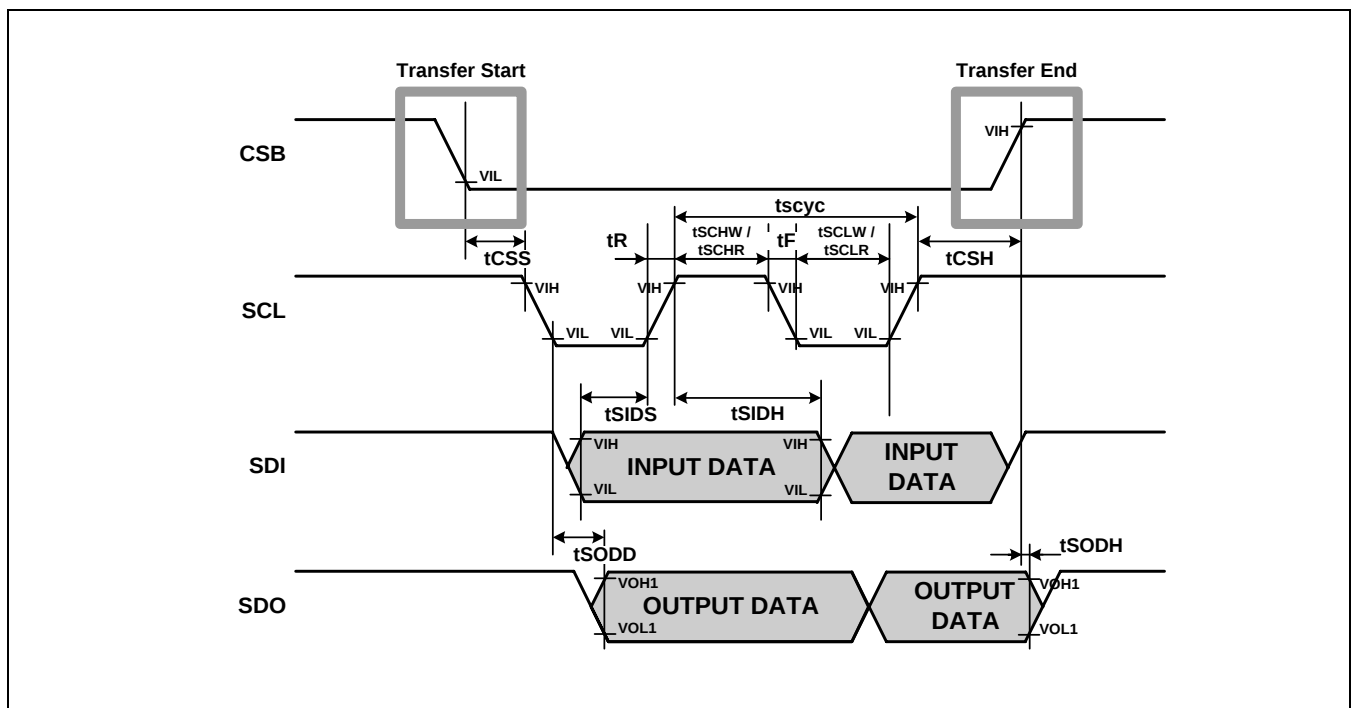
Figure 121 : AC Characteristics (SPI Mode)
