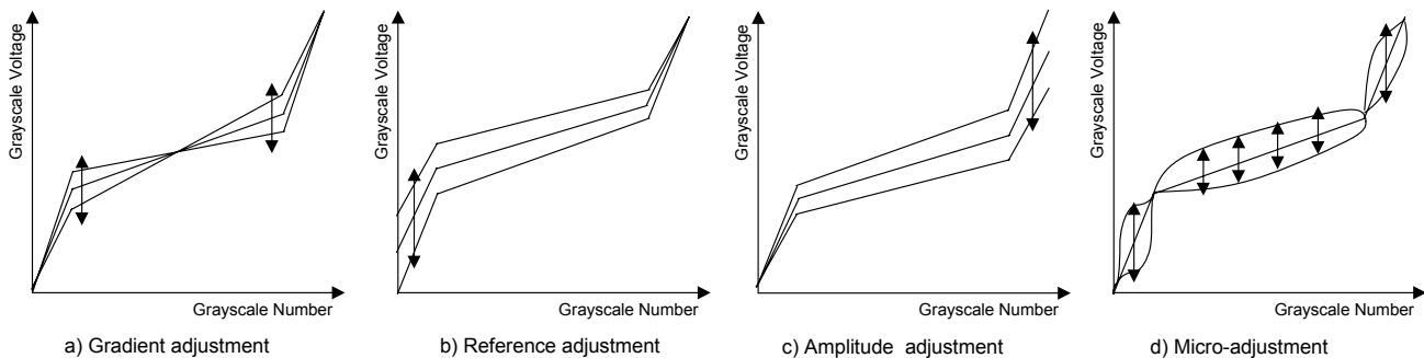
Figure 107 : The Operation of Adjusting Register
