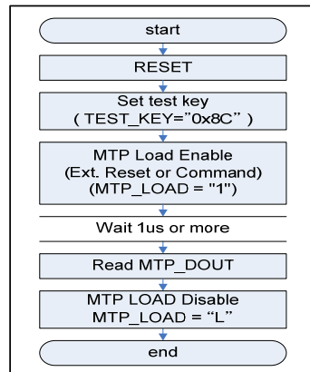
Figure 21 : Flow of MTP Load / Read
