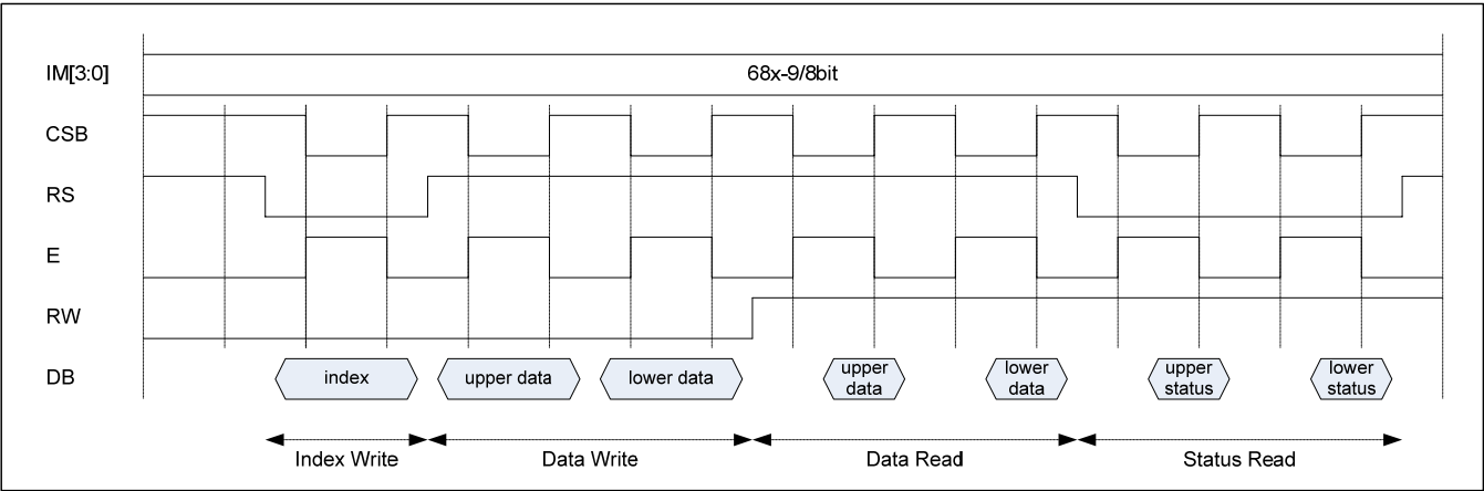
Figure 40 : Timing Diagram of 68-9bit CPU Interface
