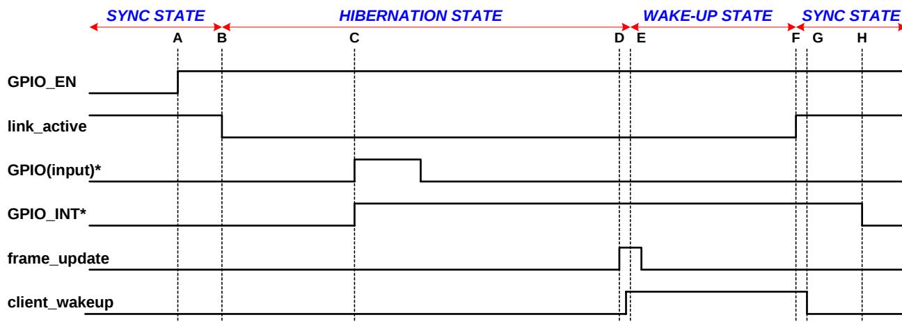
Figure 88 : GPIO based link wake-up procedure
