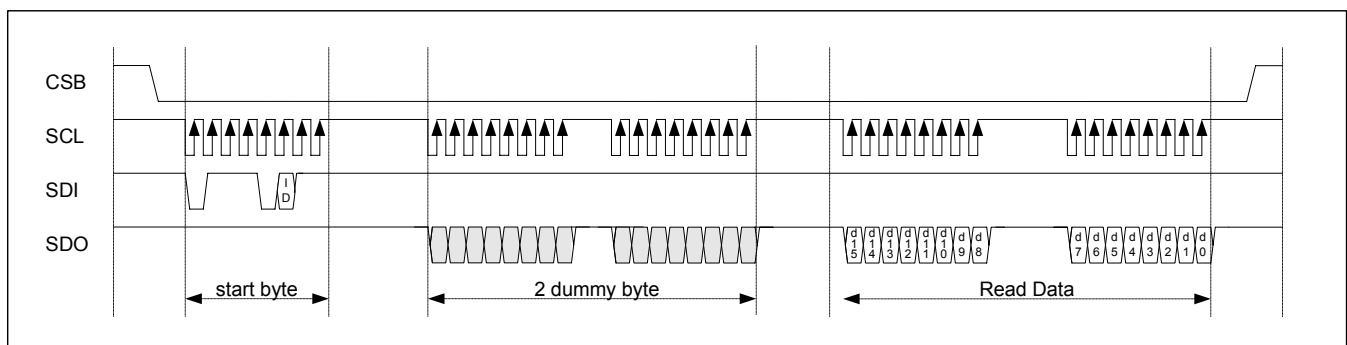
Figure 61 : Timing Diagram of GRAM-Data Read through SPI
