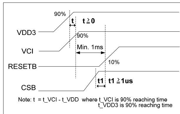
Figure 124 : External power on sequence
