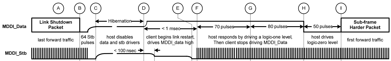
Figure 86 : Client-initiated link wake-up sequence
