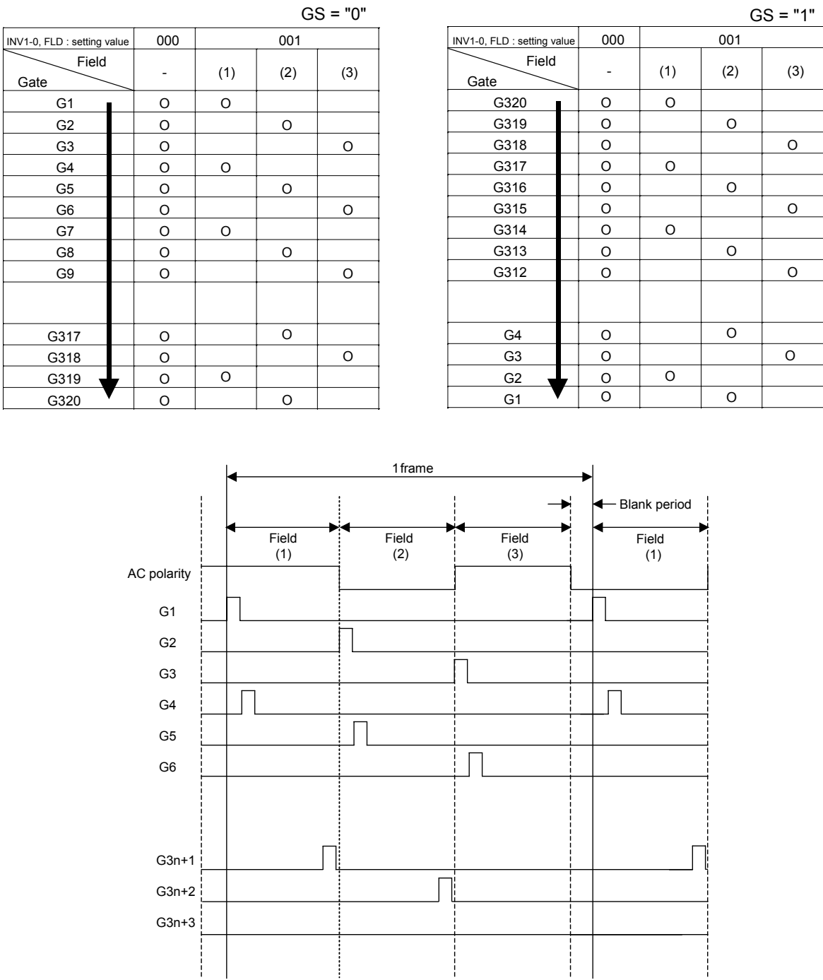
Figure 11 : Interlace drive and output waveform ( 3 Field Inversion )
