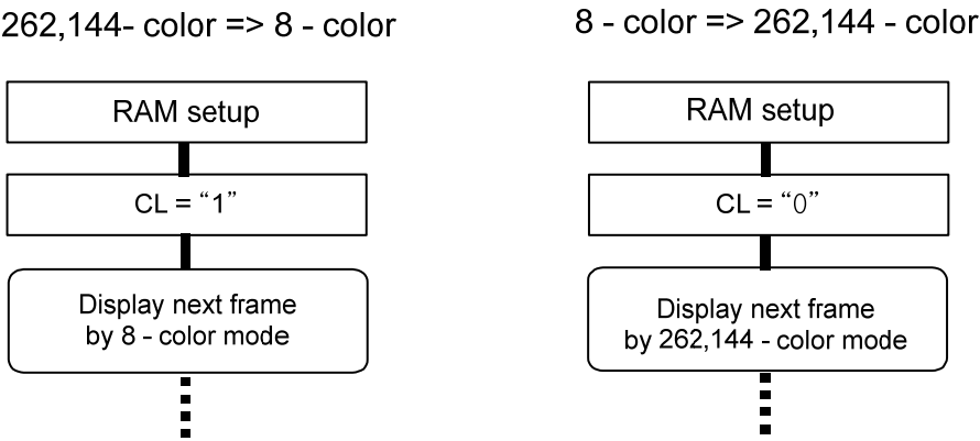
Figure 111 : Setup Procedure For The 8-Color Mode
