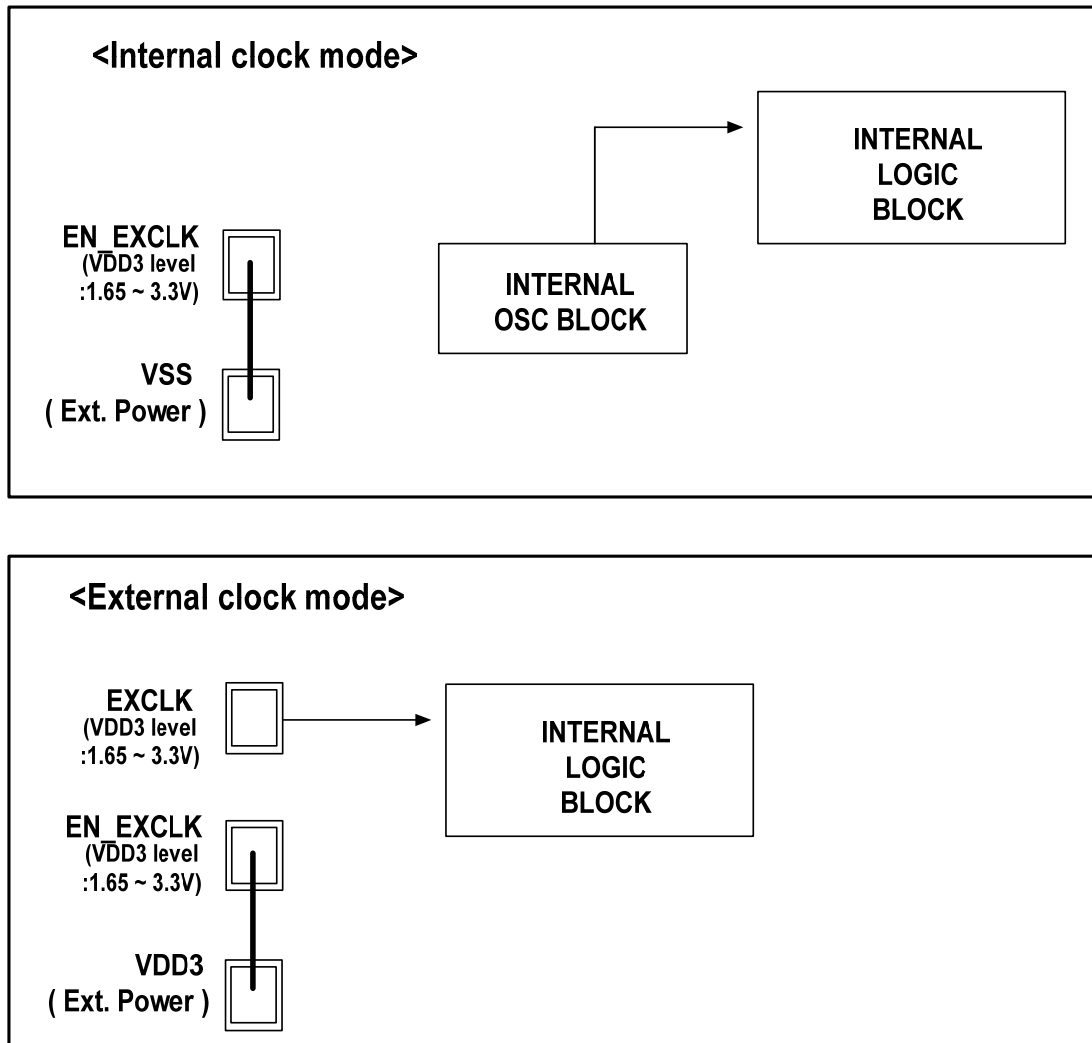
Figure 115 : Oscillation Circuit
