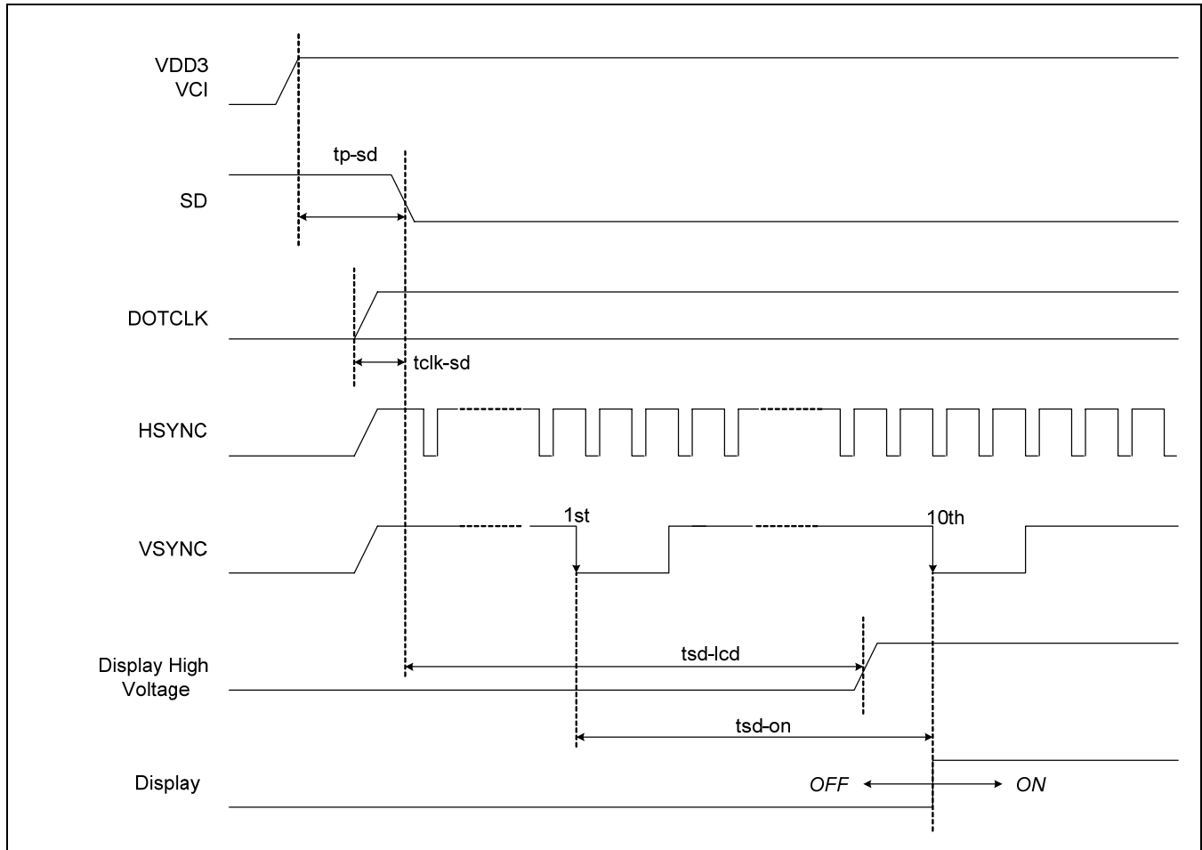
Figure 5 : Power Up Sequence Timing Diagram
