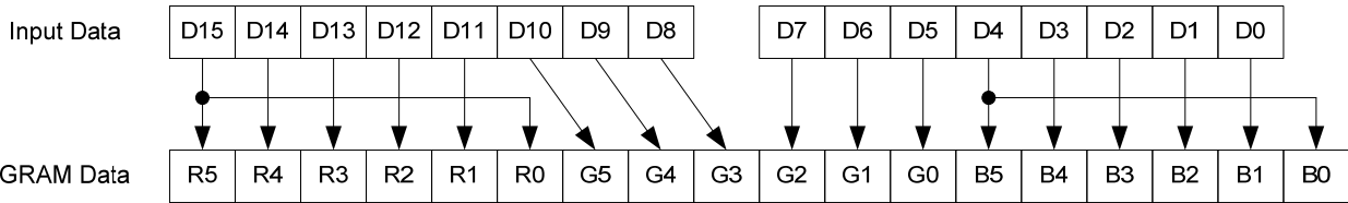
Figure 57 : Bit Assignment of GRAM Data on SPI
