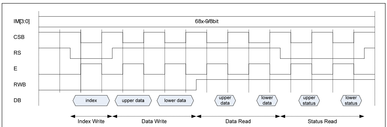
Figure 43 : Timing Diagram of 68-8bit CPU Interface
