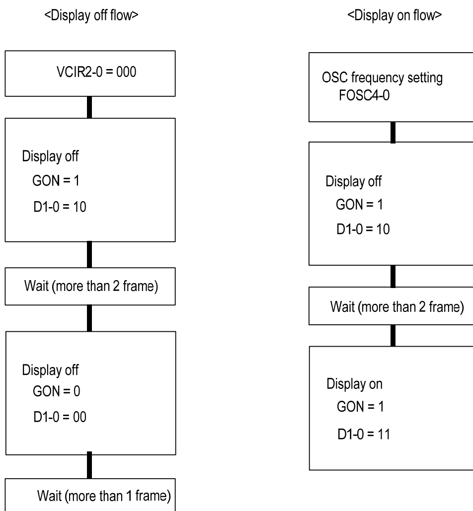
Figure 112 : DISPLAY ON / OFF SEQUENCE
