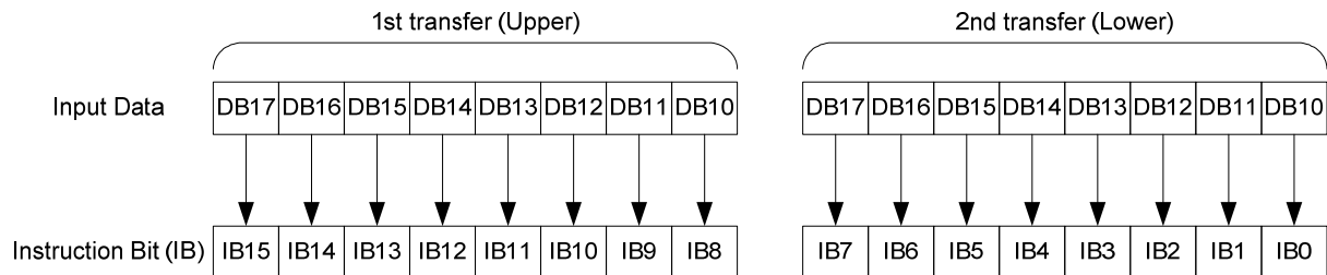
Figure 41 : Bit Assignment of Instructions on 68-8bit CPU Interface
