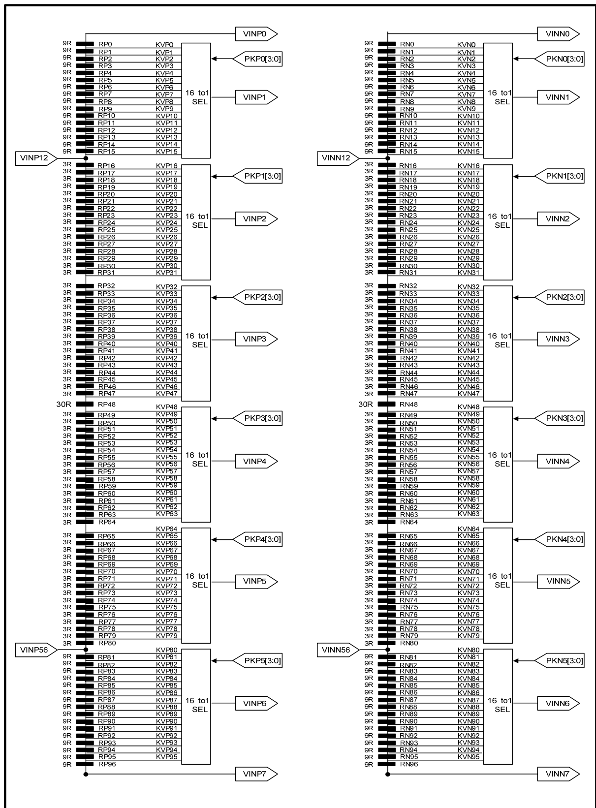
Figure 106 : Structure of Resistor Ladder Network 2
