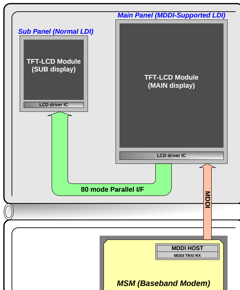
Figure 90 : Schematic diagram of sub panel control function
