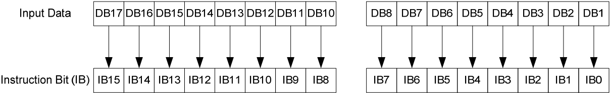
Figure 35 : Bit Assignment of Instructions on 68-16bit CPU Interface
