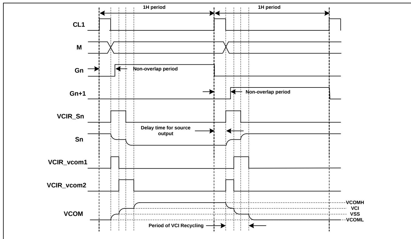
Figure 13 : Set Delay From Gate Output To Source Output And VCIR Signal
