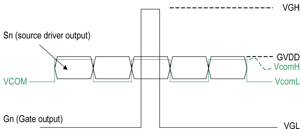
Figure 28 : Power-Up Pattern Diagram & An Example Of Source/VCOM Waveforms
