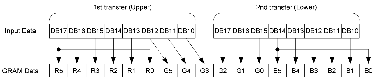
Figure 53 : Bit Assignment of Instructions on 80-8bit CPU Interface
