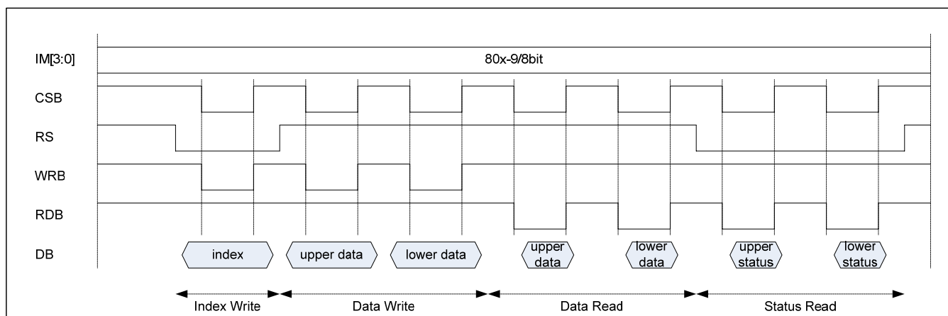
Figure 55 : Timing Diagram of 80-8bit CPU Interface
