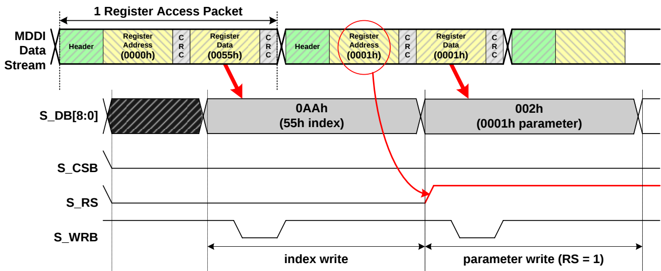
Figure 96 : 80 mode STN type included parameter
