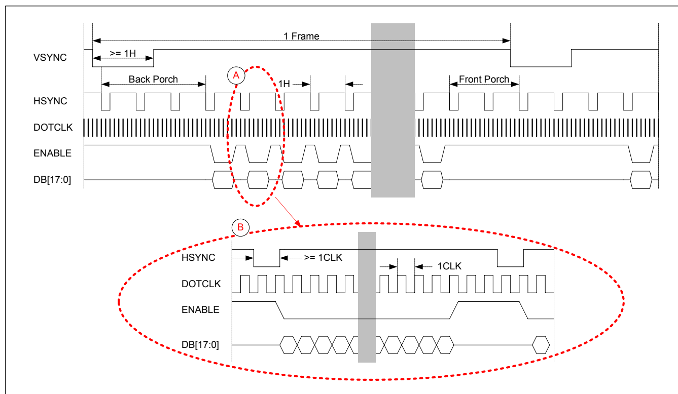
Figure 64 : Timing Diagram of 18/16bit RGB Interface
