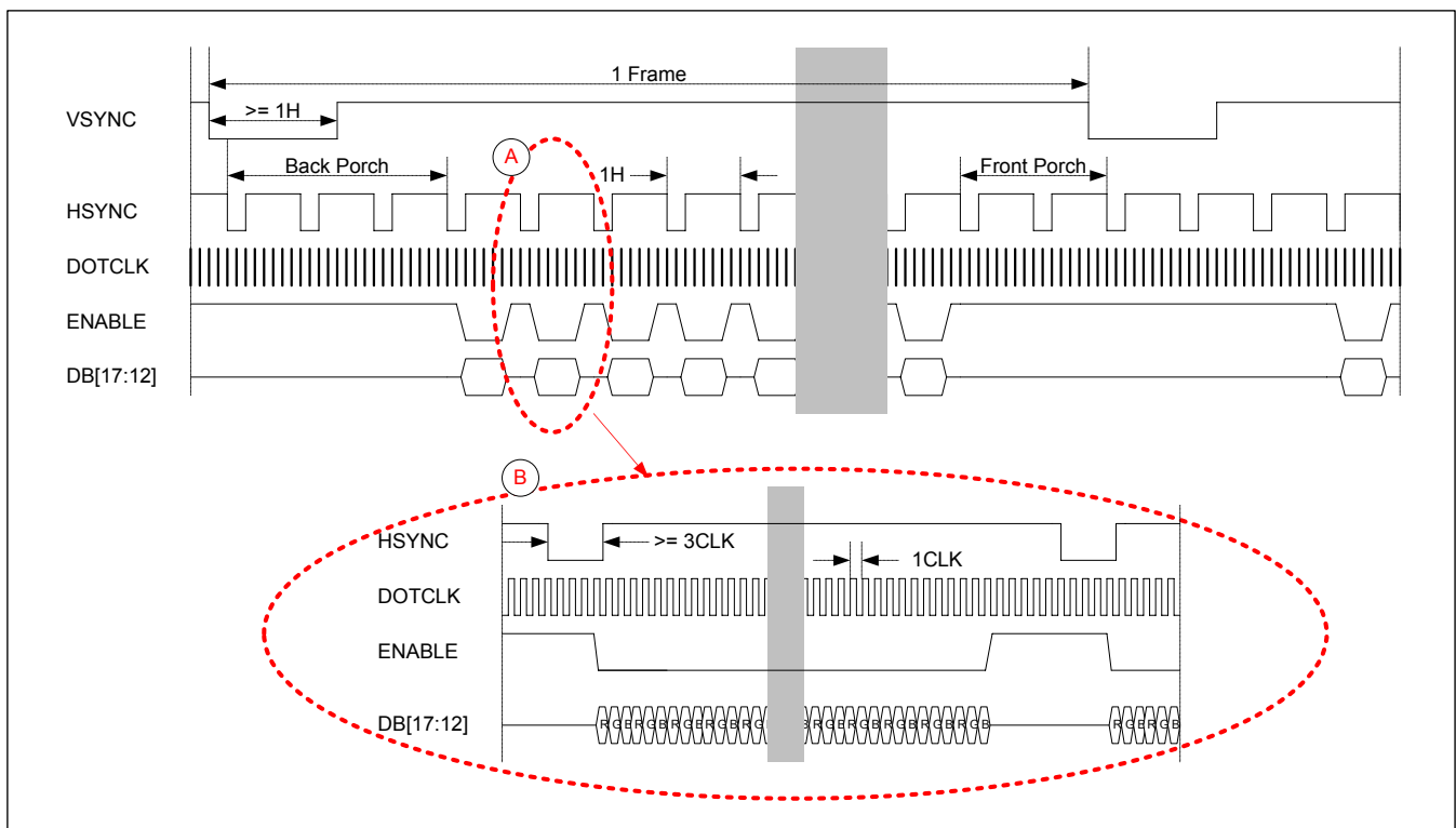
Figure 68 : Timing Diagram of 6bit RGB Interface
