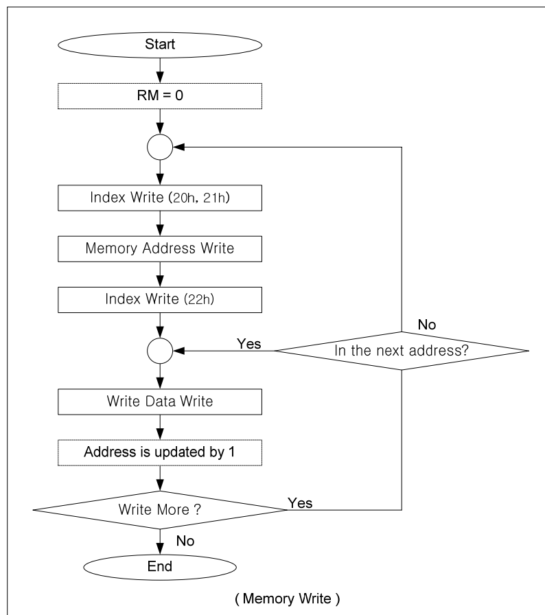
Figure 14 : Memory Data Write Sequence
