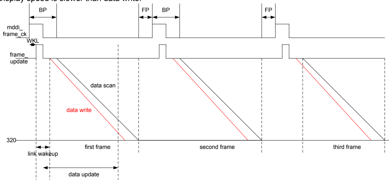
Figure 82 : Tearing-less display: data write speed is faster than display
