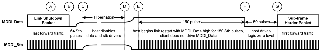
Figure 85 : Host-initiated link wakeup sequence
