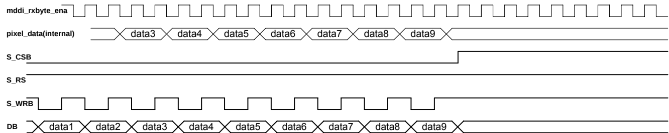
Figure 101 : Change data path timing diagram
