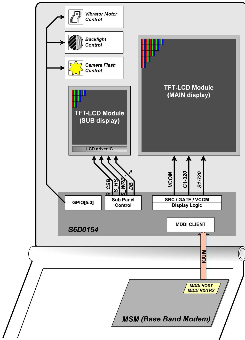
Figure 102 : MDDI-integrated system structure
