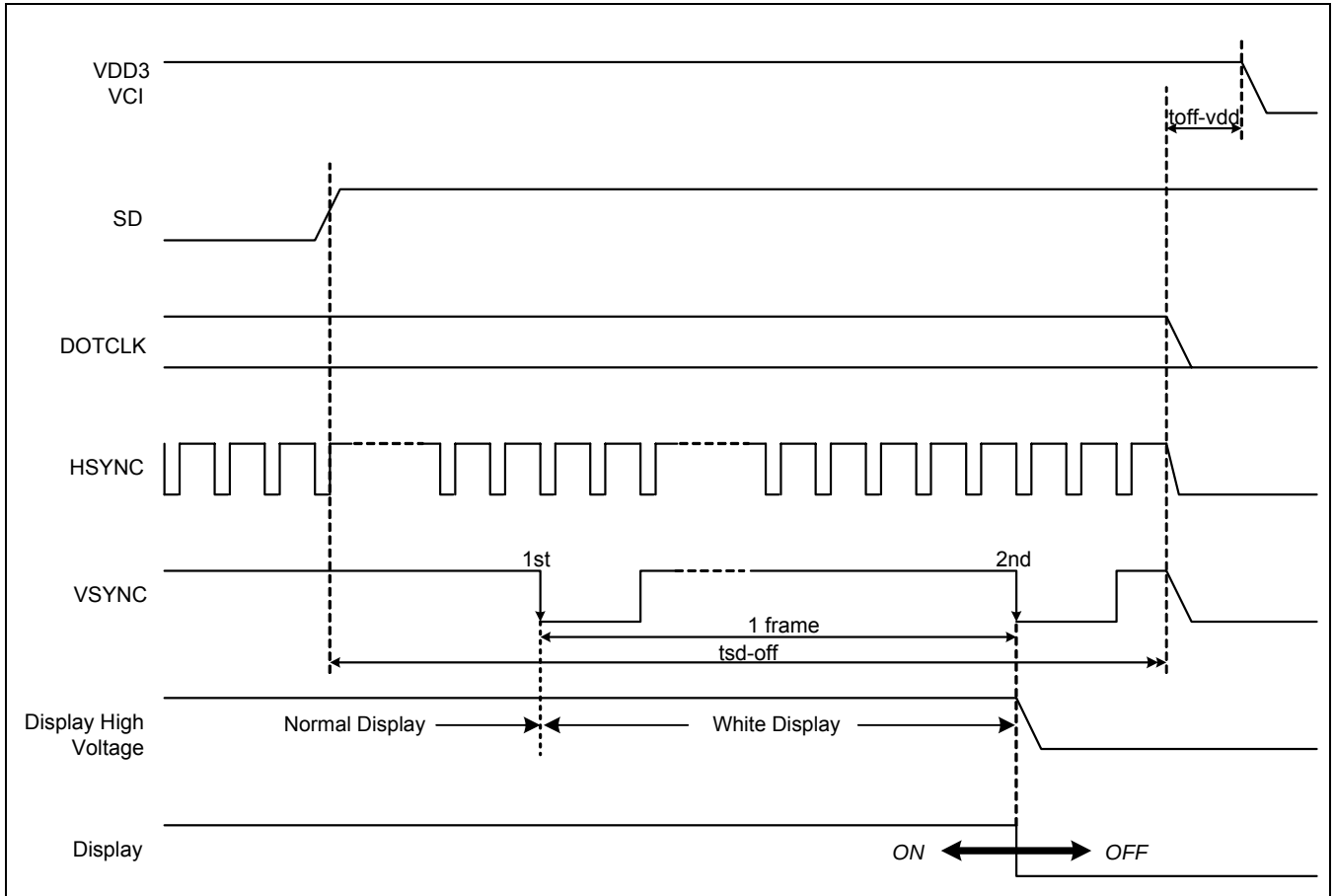
Figure 6 : Power Down Sequence Timing Diagram
