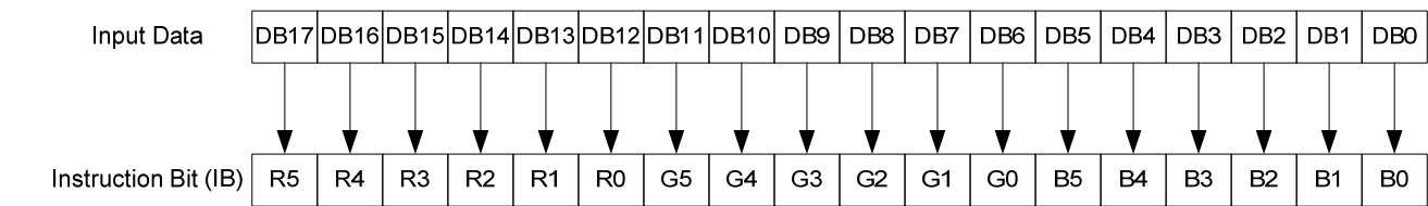
Figure 44 : Bit Assignment of Instructions on 80-18bit CPU Interface
