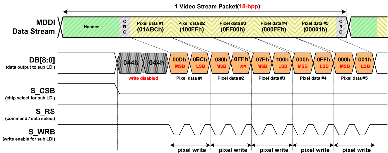
Figure 97 : 80 mode STN type 9 bit video data transfer
