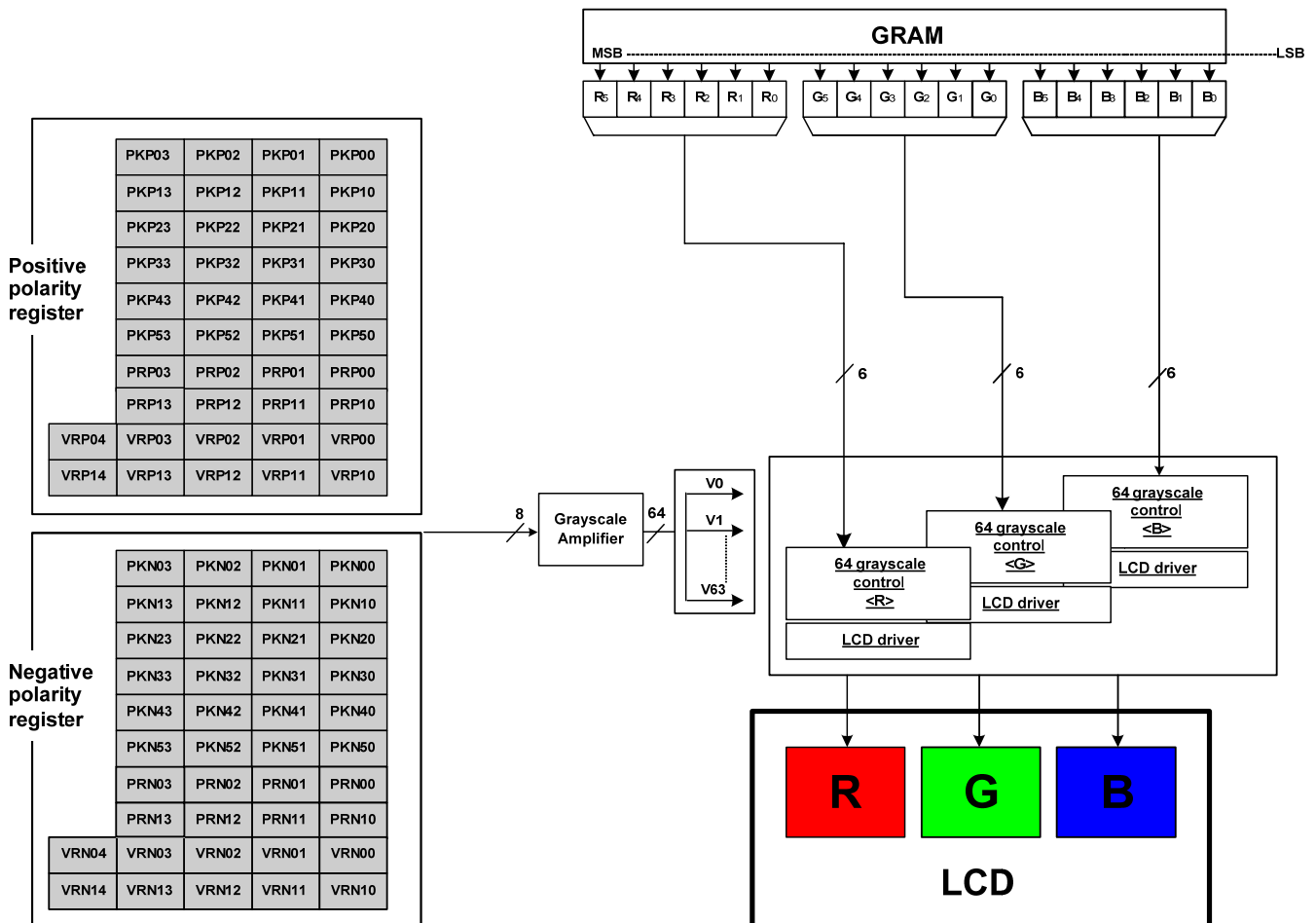
Figure 103 : Grayscale Control
