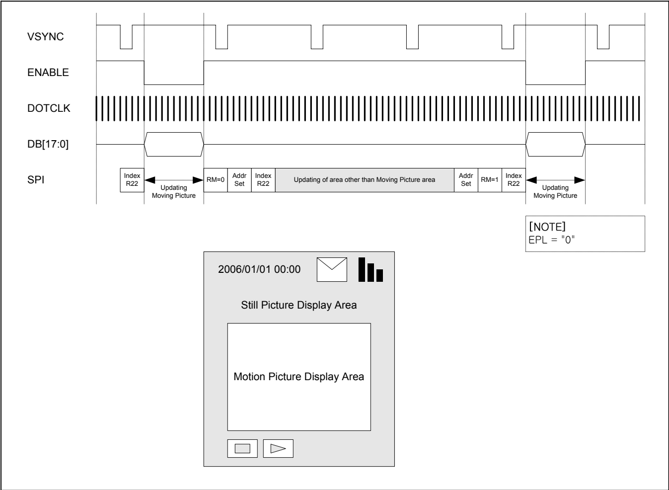
Figure 70 : GRAM Access through RGB Interface and SPI
