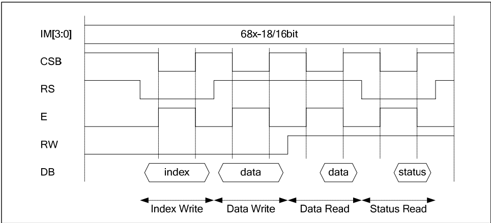
Figure 37 : Timing Diagram of 68-16bit CPU Interface
